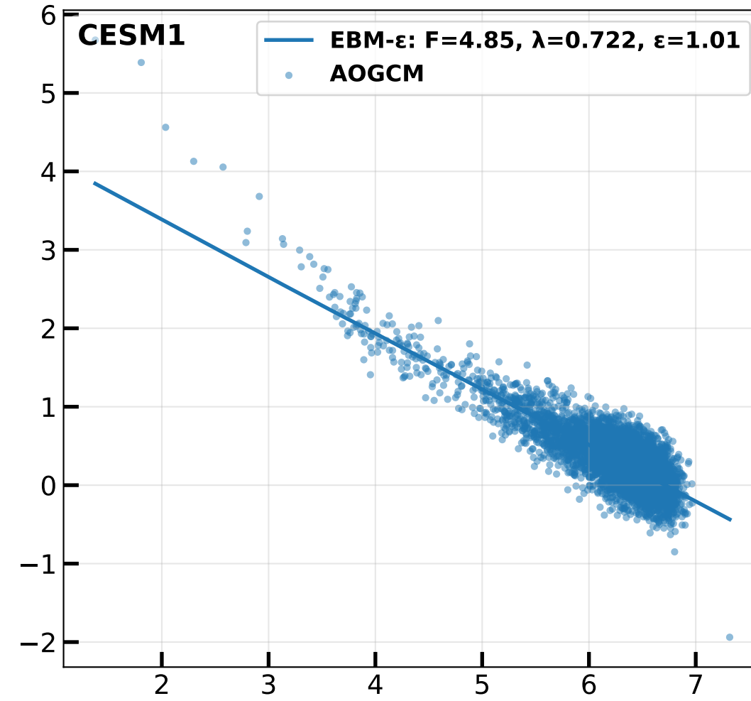
4xCO 2 Net TOA vs T 2M (radiative fit, iter 7)
