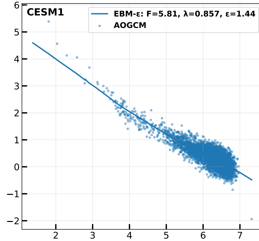
4xCO 2 Net TOA vs T 2M (radiative fit, iter 4)
