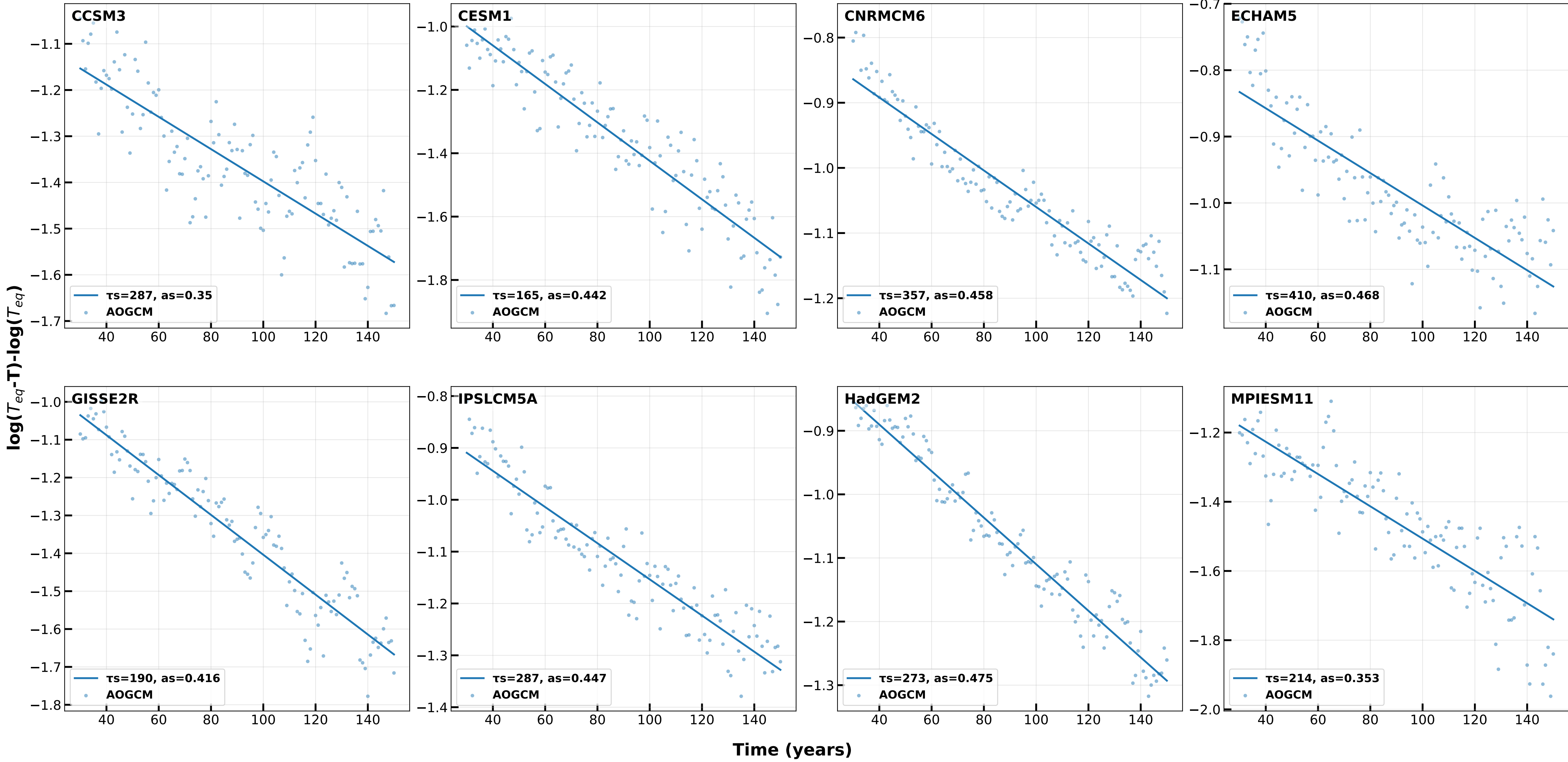
4xCO 2 log(T eq -T) - log(T eq ) vs. Time (slow mode, iter 1)
