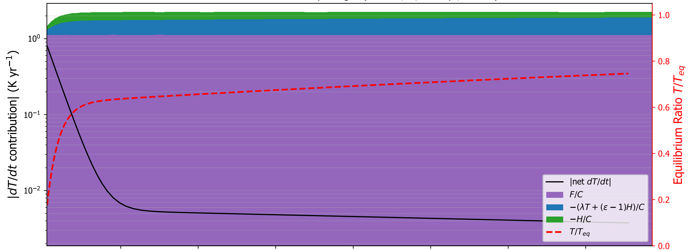
CCSM3: surface tendency budget ( \varepsilon=0.83 , \tau_s=367 yr, C=3.9 )
