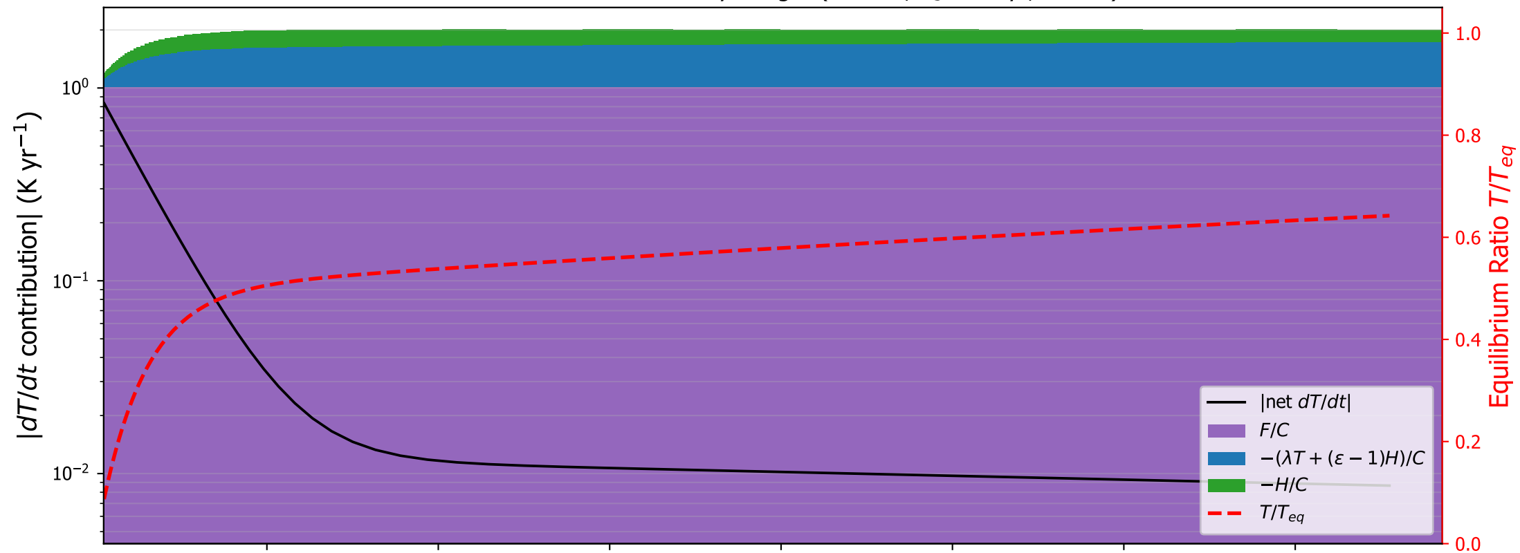
CNRMCM6: surface tendency budget ( \varepsilon=1.29 , \tau_s=435 yr, C=7.6 )
