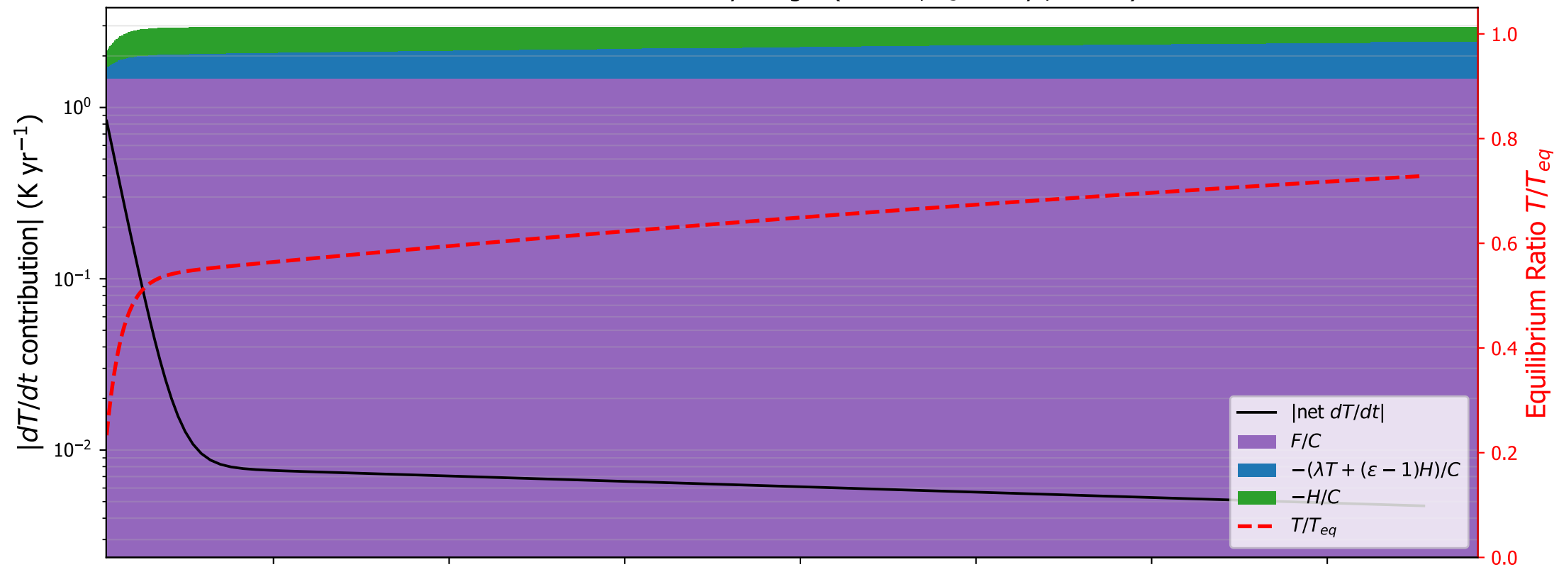
GISSE2R: surface tendency budget ( \varepsilon=0.74 , \tau_s=276 yr, C=2.8 )
