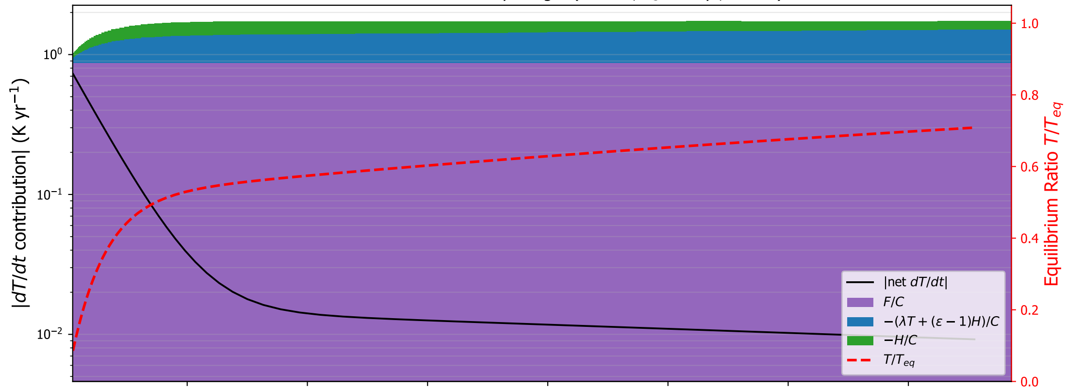
HadGEM2: surface tendency budget ( \varepsilon=1.10 , \tau_s=294 yr, C=7.1 )
