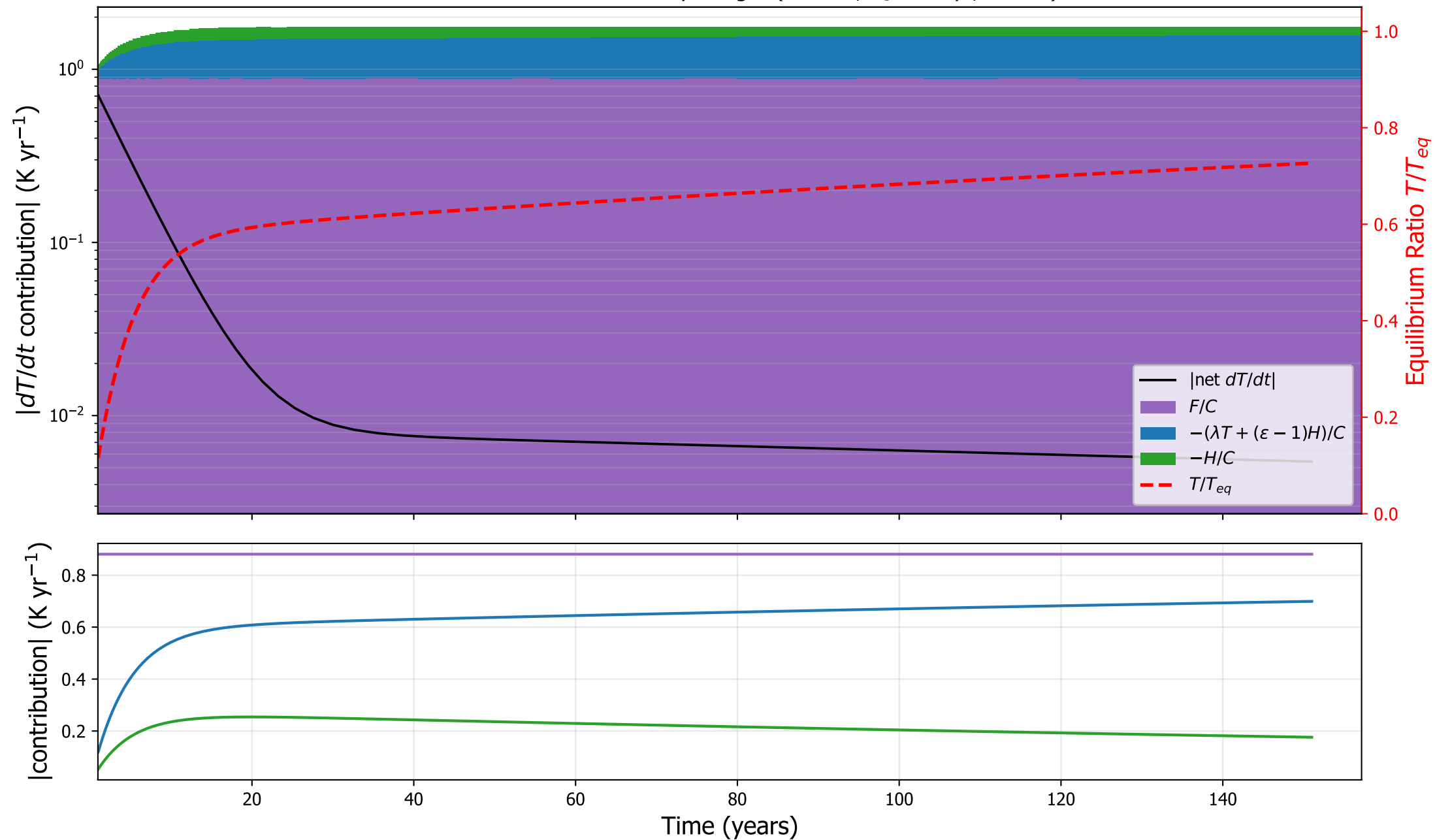
MPIESM11: surface tendency budget ( \varepsilon=1.34 , \tau_s=345 yr, C=9.0 )
