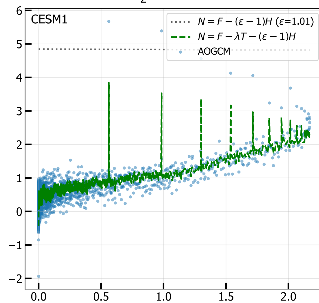
4xCO 2 Net TOA vs Ocean Heat Uptake H (radiative fit, iter 9)
