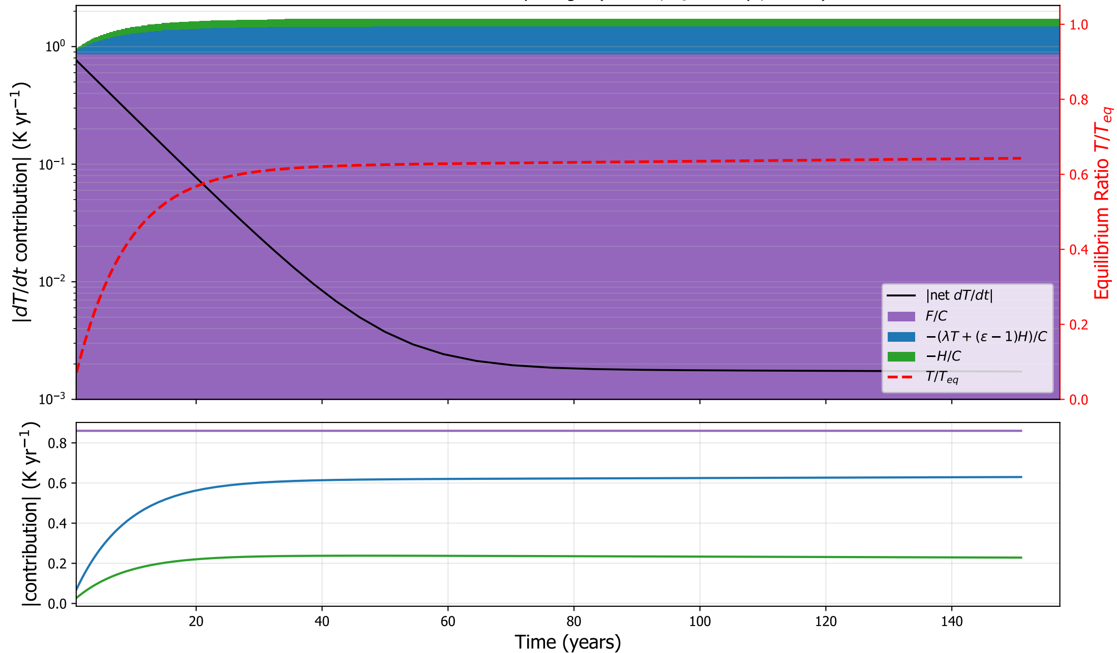
CNRMCM6: surface tendency budget ( \varepsilon=1.34 , \tau_s=2358 yr, C=8.0 )
