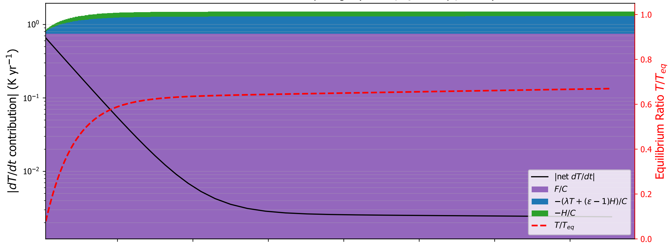
IPSLCM5A: surface tendency budget ( \varepsilon=1.27 , \tau_s=1223 yr, C=8.6 )
