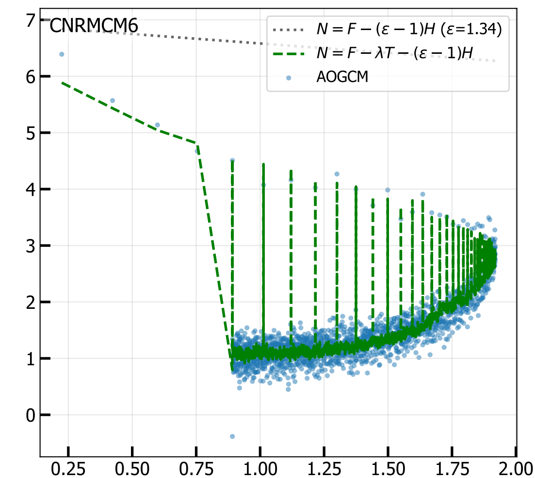
4xCO 2 Net TOA vs Ocean Heat Uptake H (radiative fit, iter 4)
