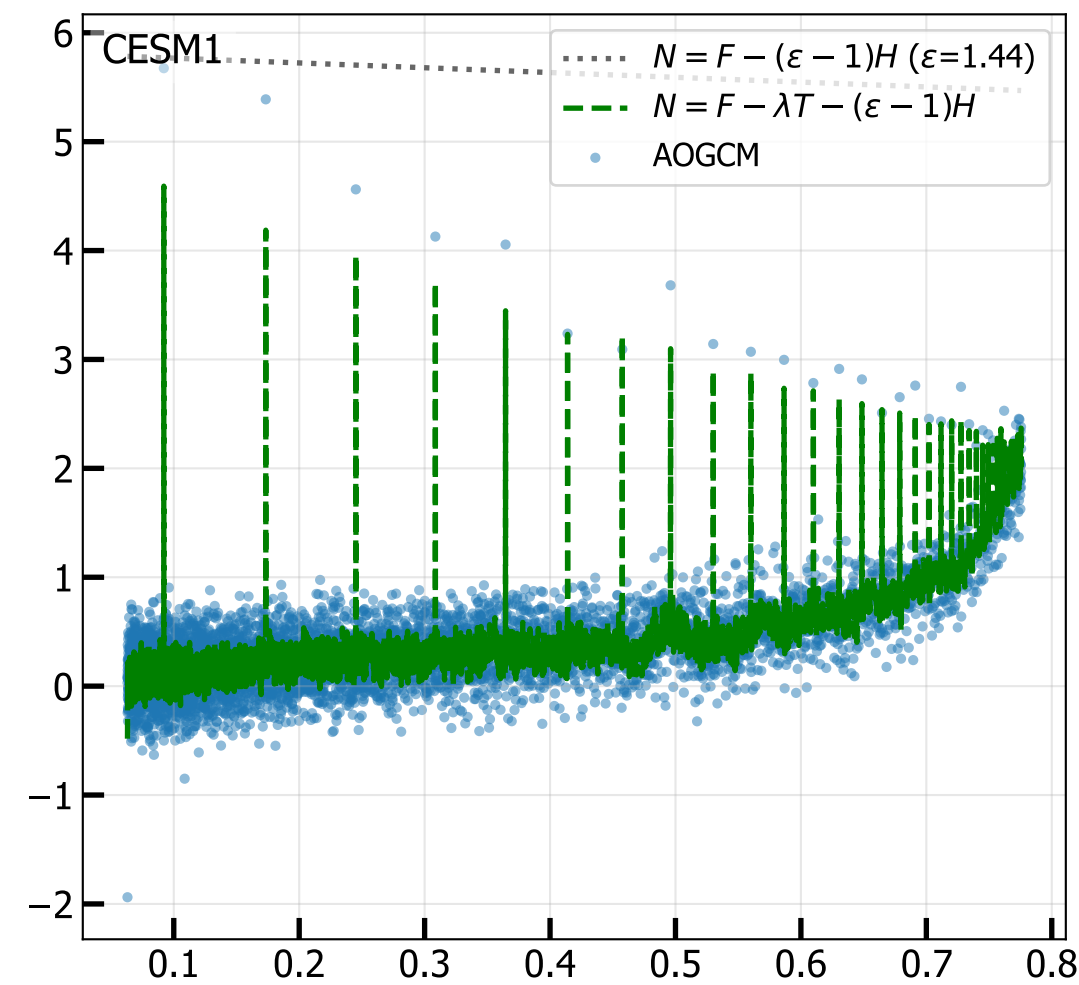
4xCO 2 Net TOA vs Ocean Heat Uptake H (radiative fit, iter 5)
