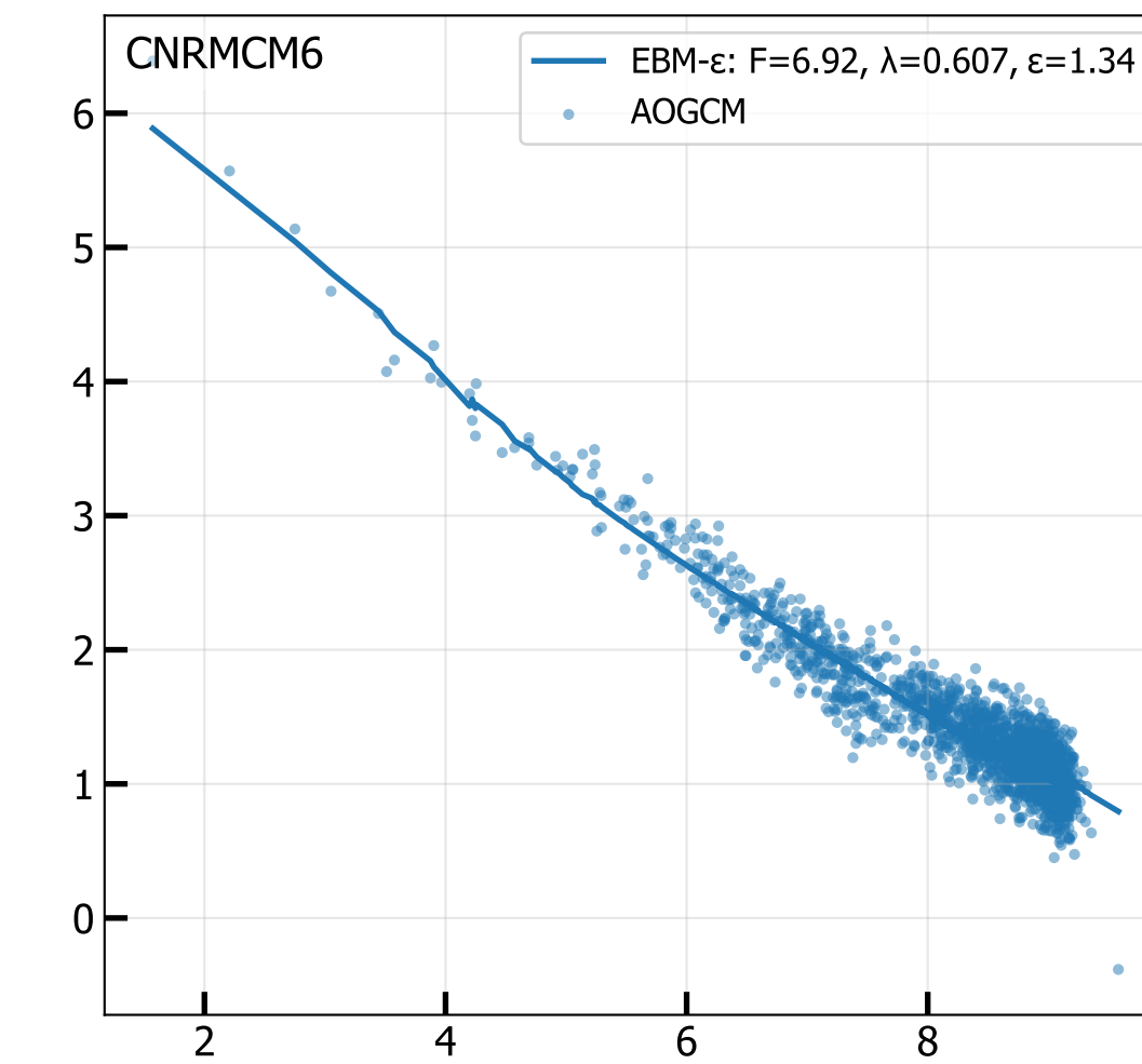
4xCO 2 Net TOA vs T 2M (radiative fit, iter 8)
