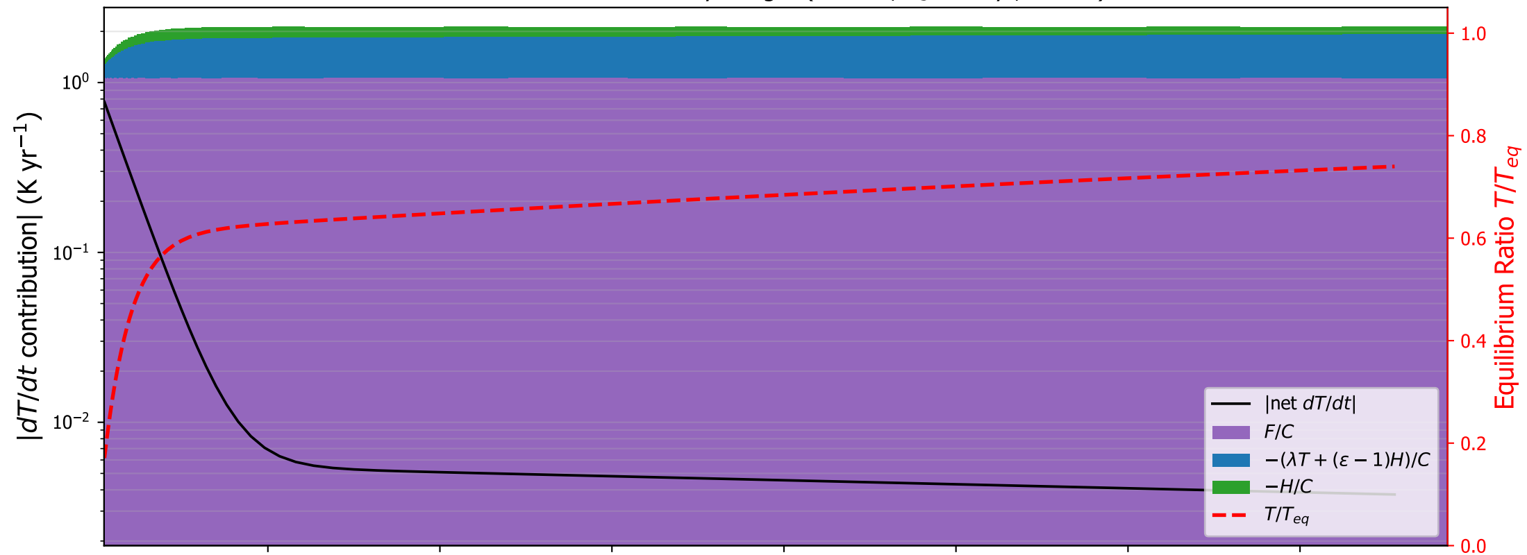
CCSM3: surface tendency budget ( \varepsilon=1.38 , \tau_s=368 yr, C=6.8 )
