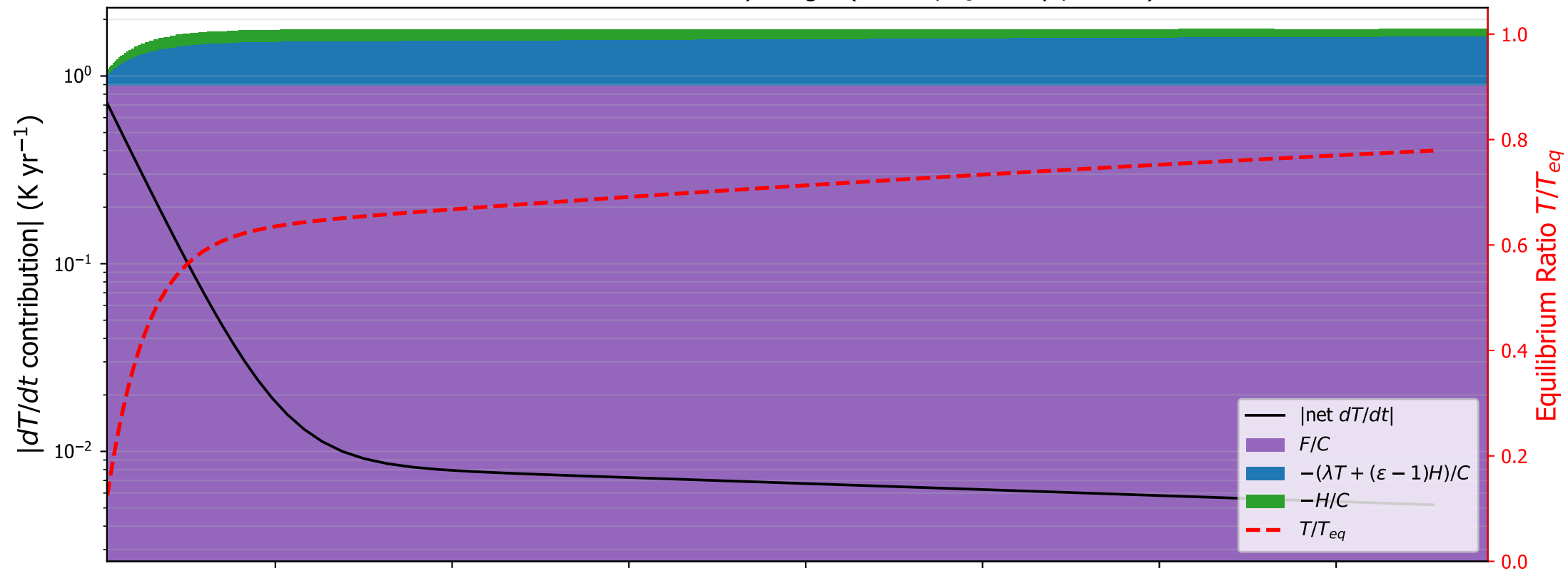
MPIESM11: surface tendency budget ( \varepsilon=1.27 , \tau_s=272 yr, C=9.9 )
