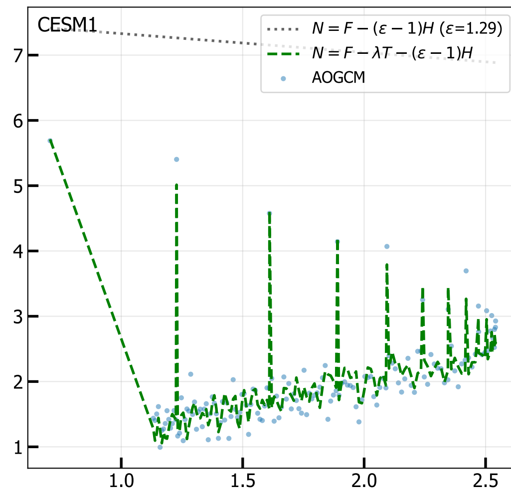
4xCO 2 Net TOA vs Ocean Heat Uptake H (radiative fit, iter 2)
