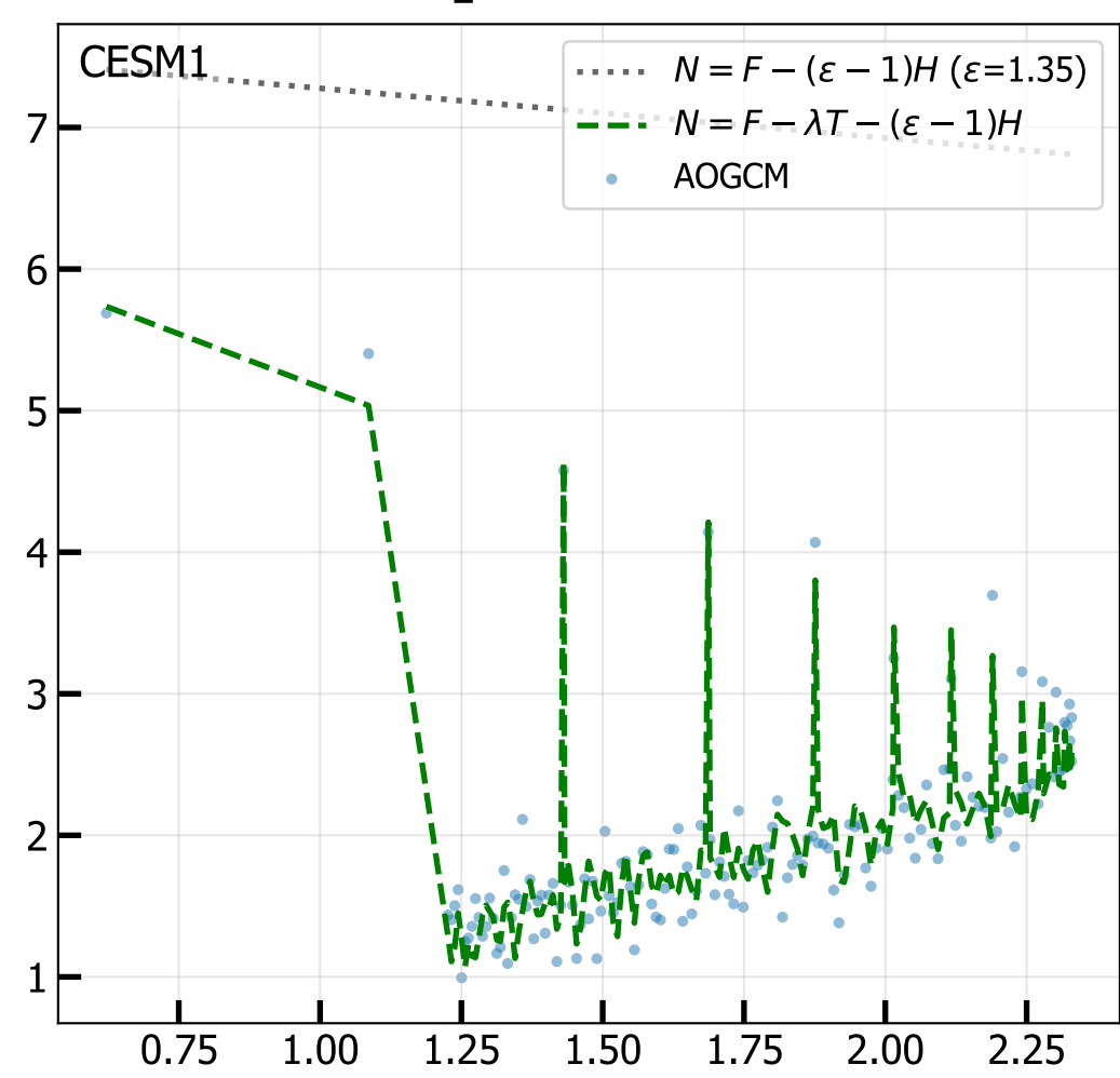
4xCO 2 Net TOA vs Ocean Heat Uptake H (radiative fit, iter 10)
