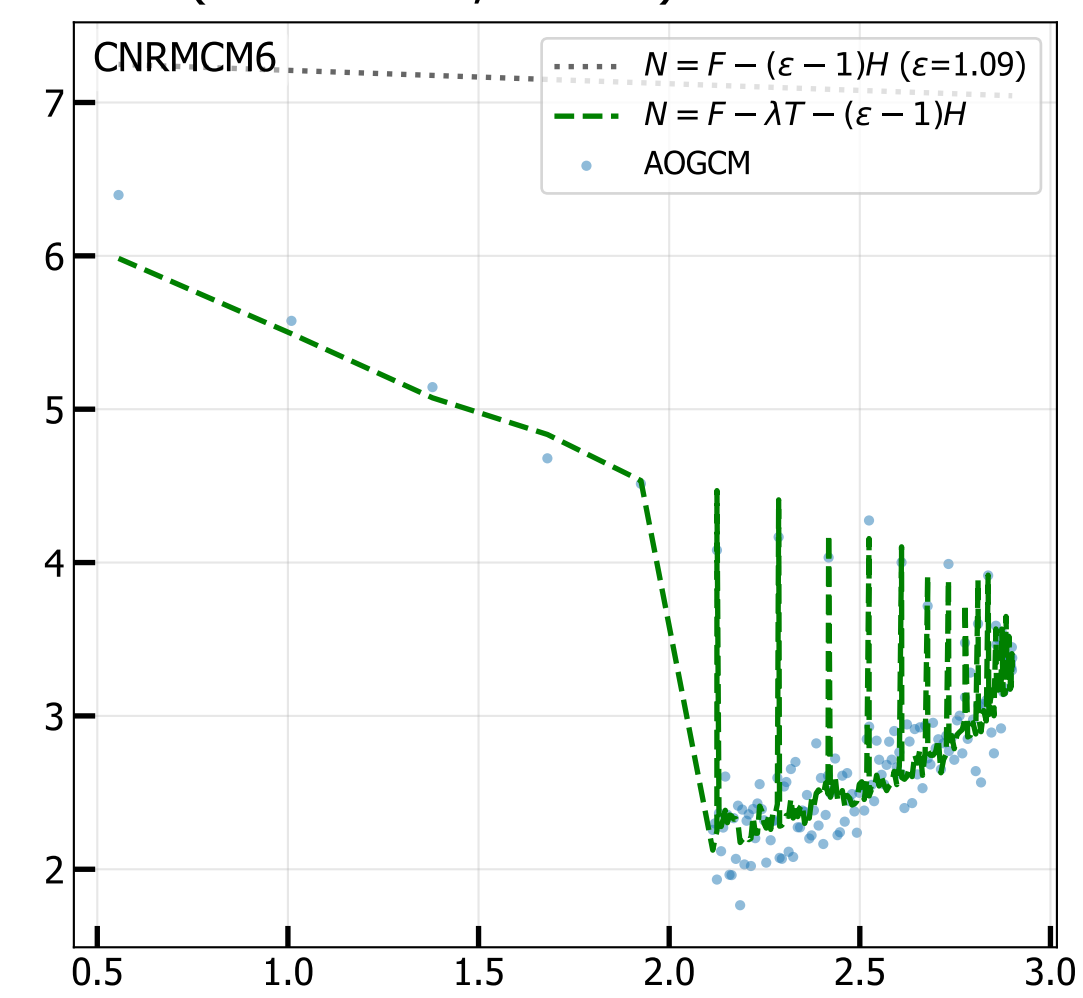
4xCO 2 Net TOA vs Ocean Heat Uptake H (radiative fit, iter 10)
