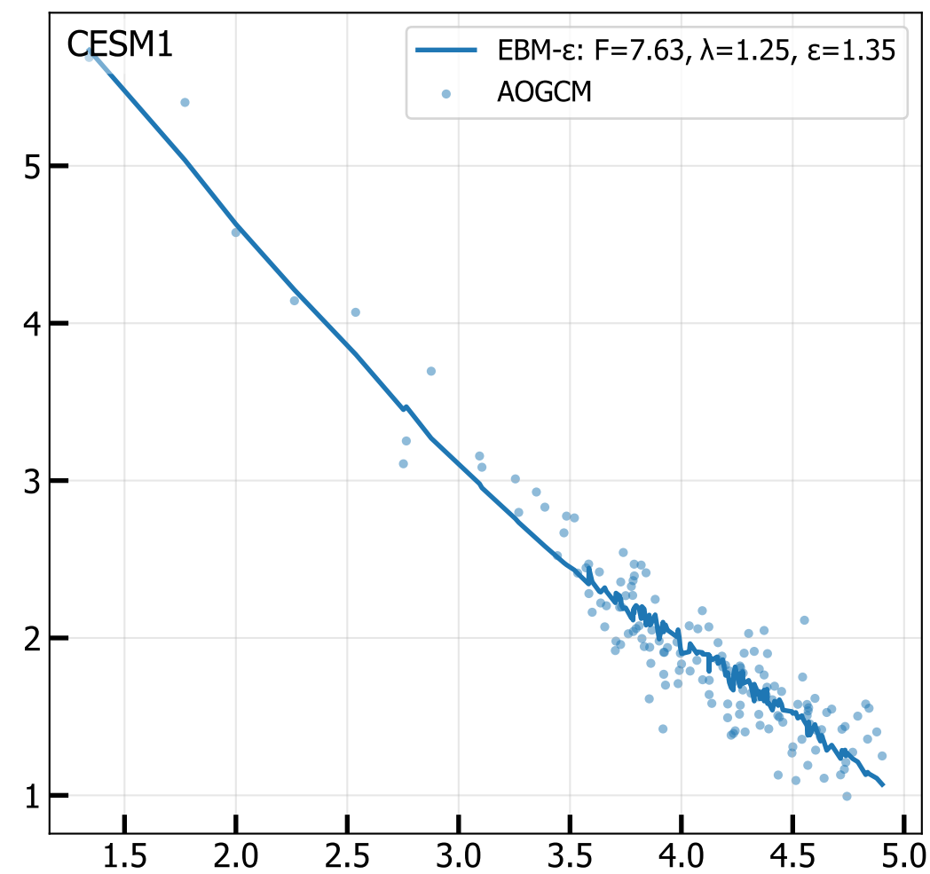
4xCO 2 Net TOA vs T 2M (radiative fit, iter 10)
