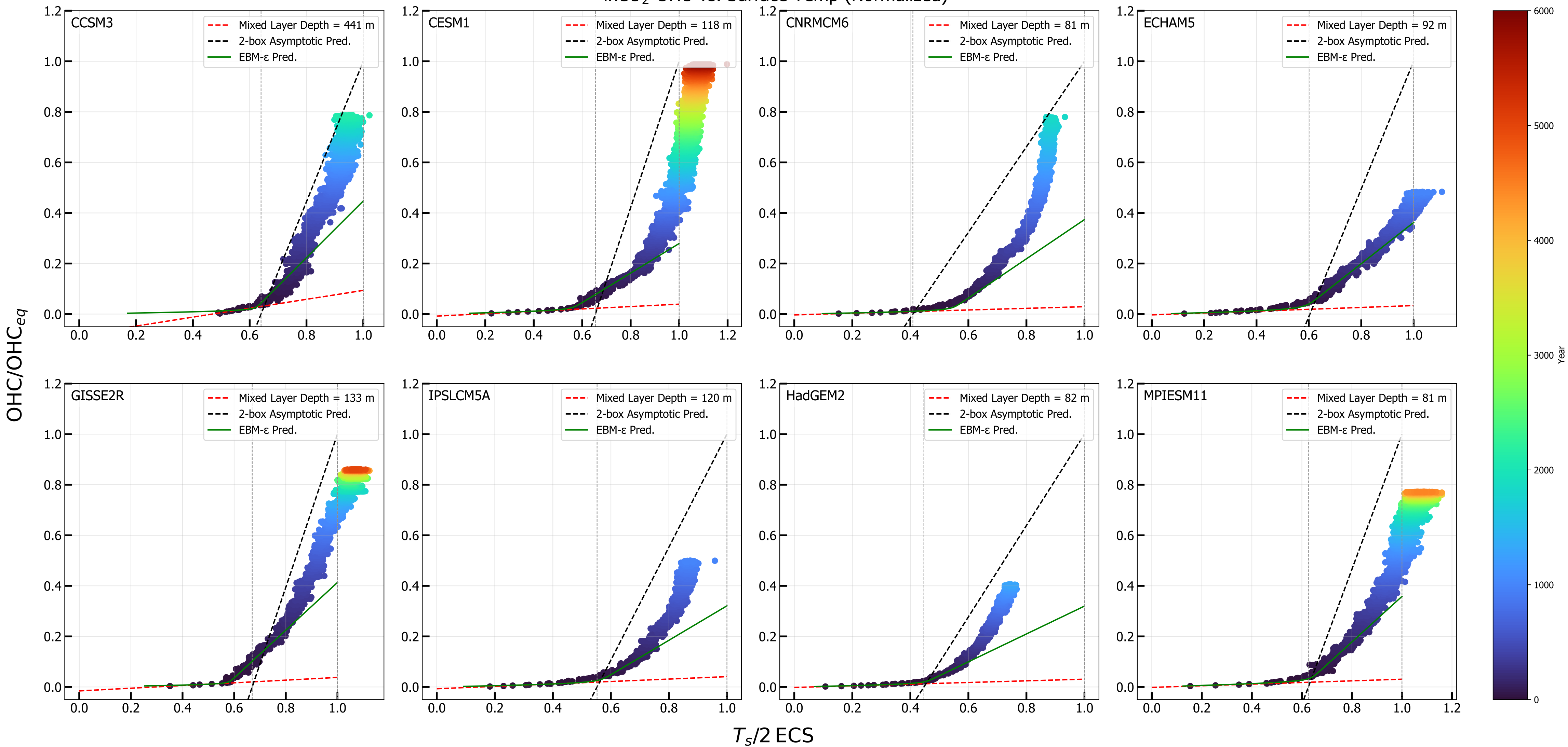
4xCO 2 OHU vs. Surface Temp (Normalized)
