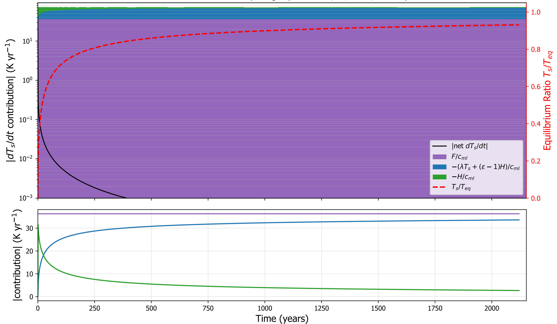
CCSM3: surface tendency budget ( \kappa=5.6\text{e-}05 , h_{ml}=1 m, \varepsilon=0.92 )
