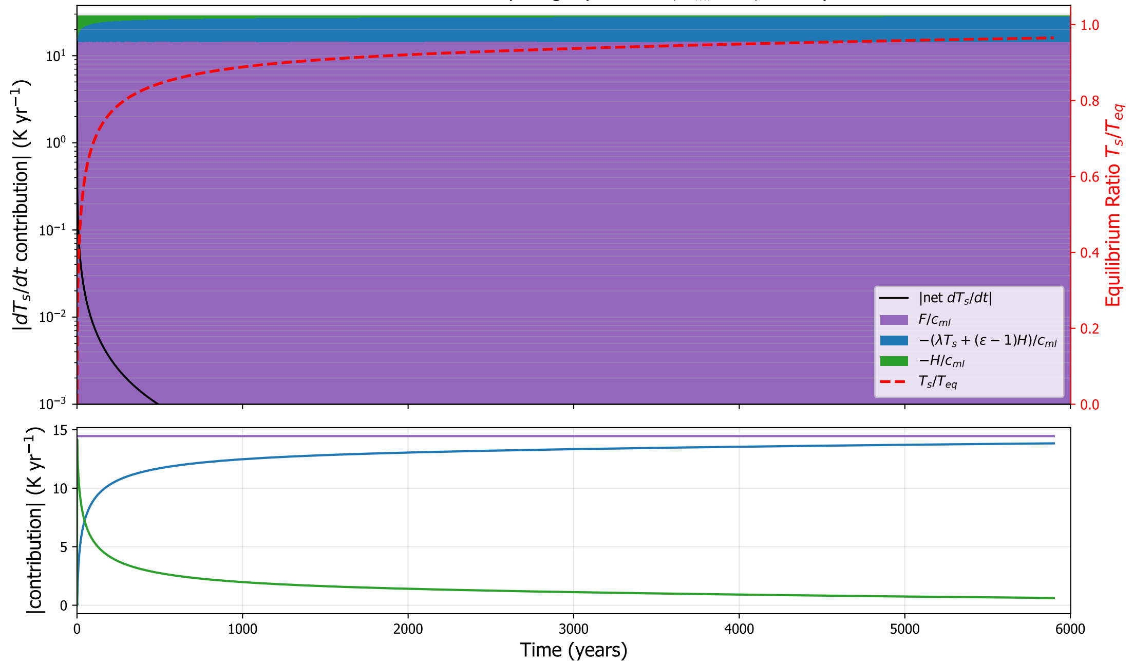
CESM1: surface tendency budget ( \kappa=4.6\text{e-}05 , h_{ml}=2 m, \varepsilon=0.82 )
