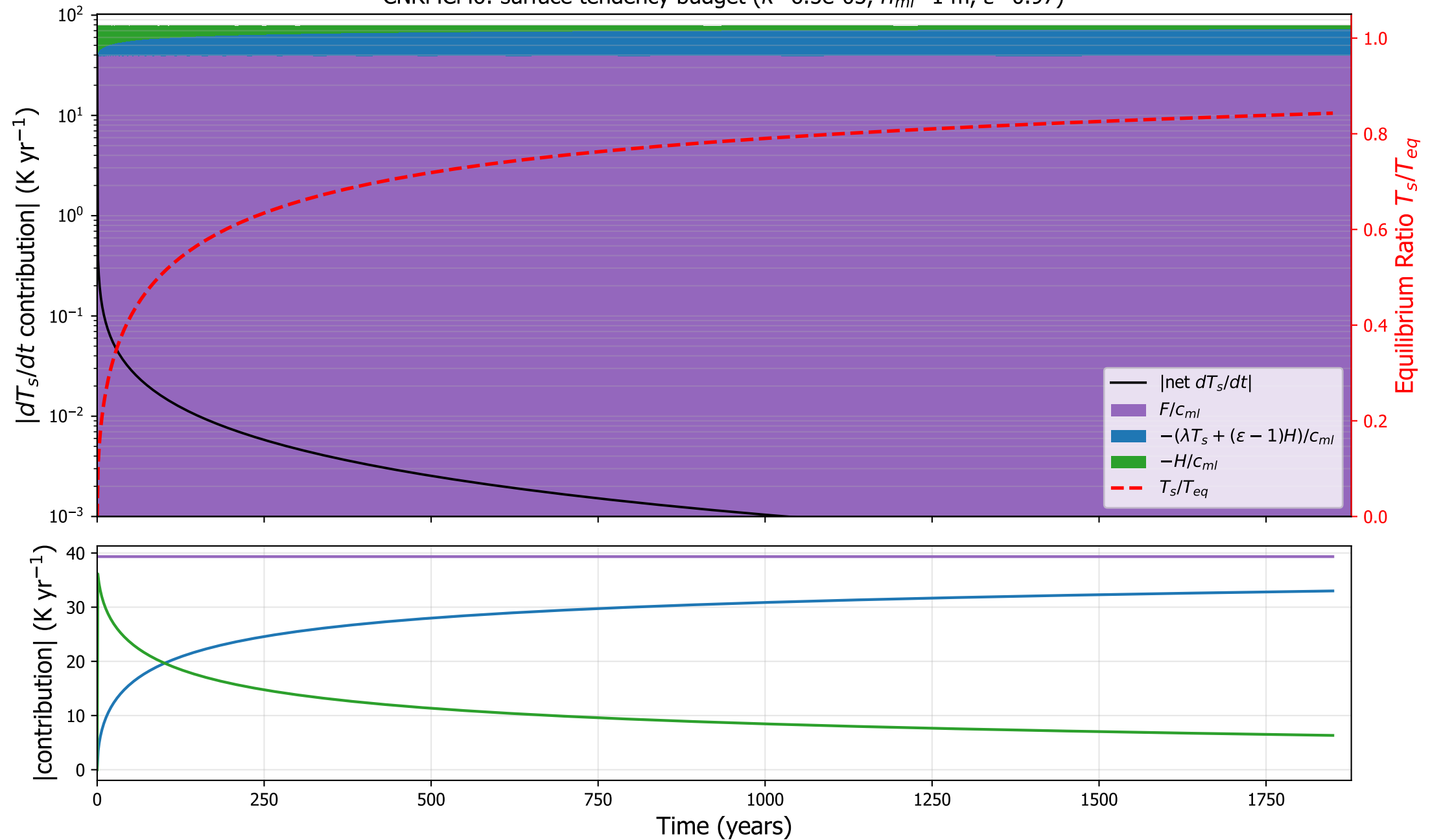
CNRMCM6: surface tendency budget ( \kappa=6.5\text{e-}05 , h_{ml}=1 m, \varepsilon=0.97 )
