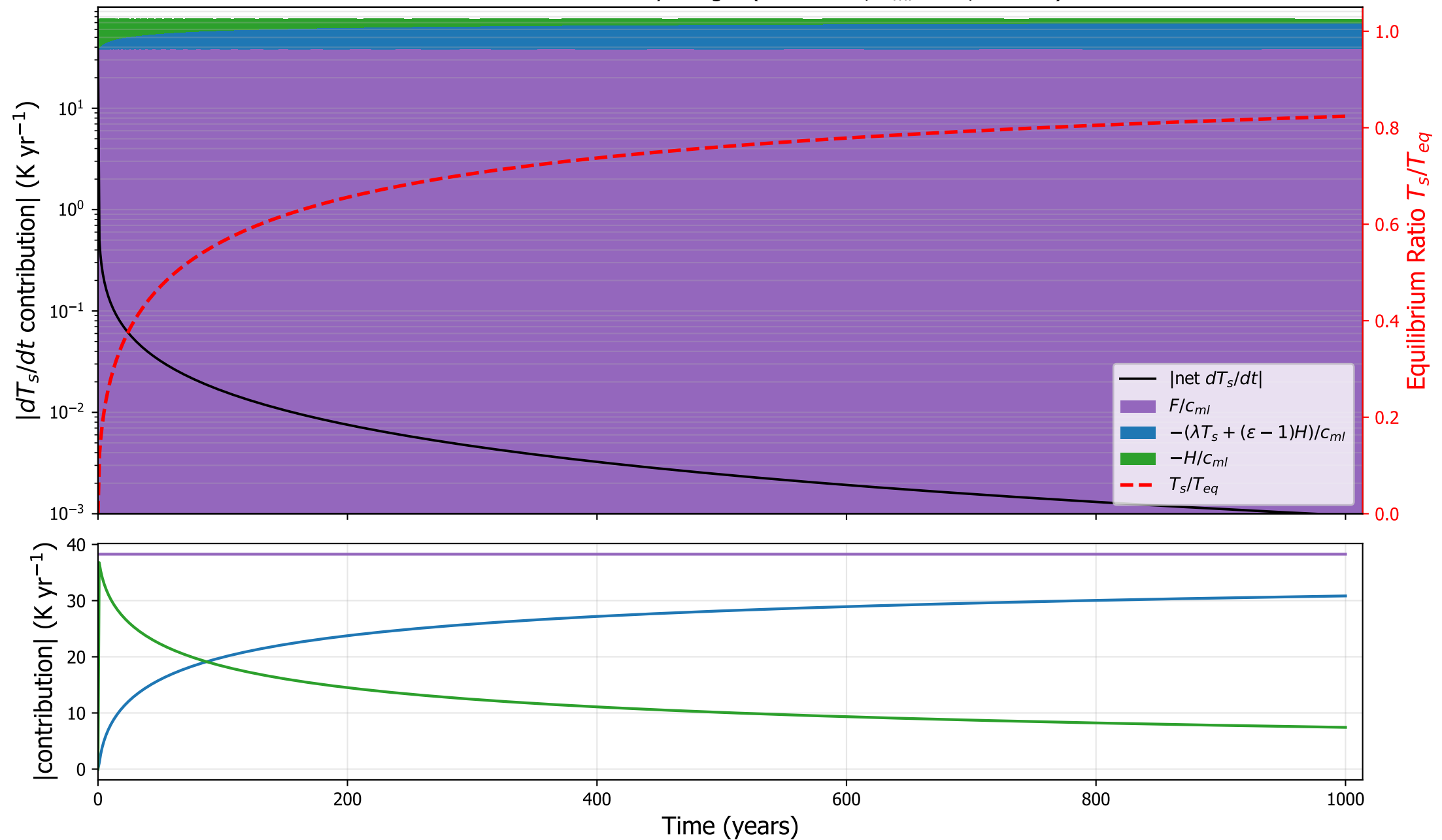
ECHAM5: surface tendency budget ( \kappa=4.2\text{e-}05 , h_{ml}=1 m, \varepsilon=0.91 )
