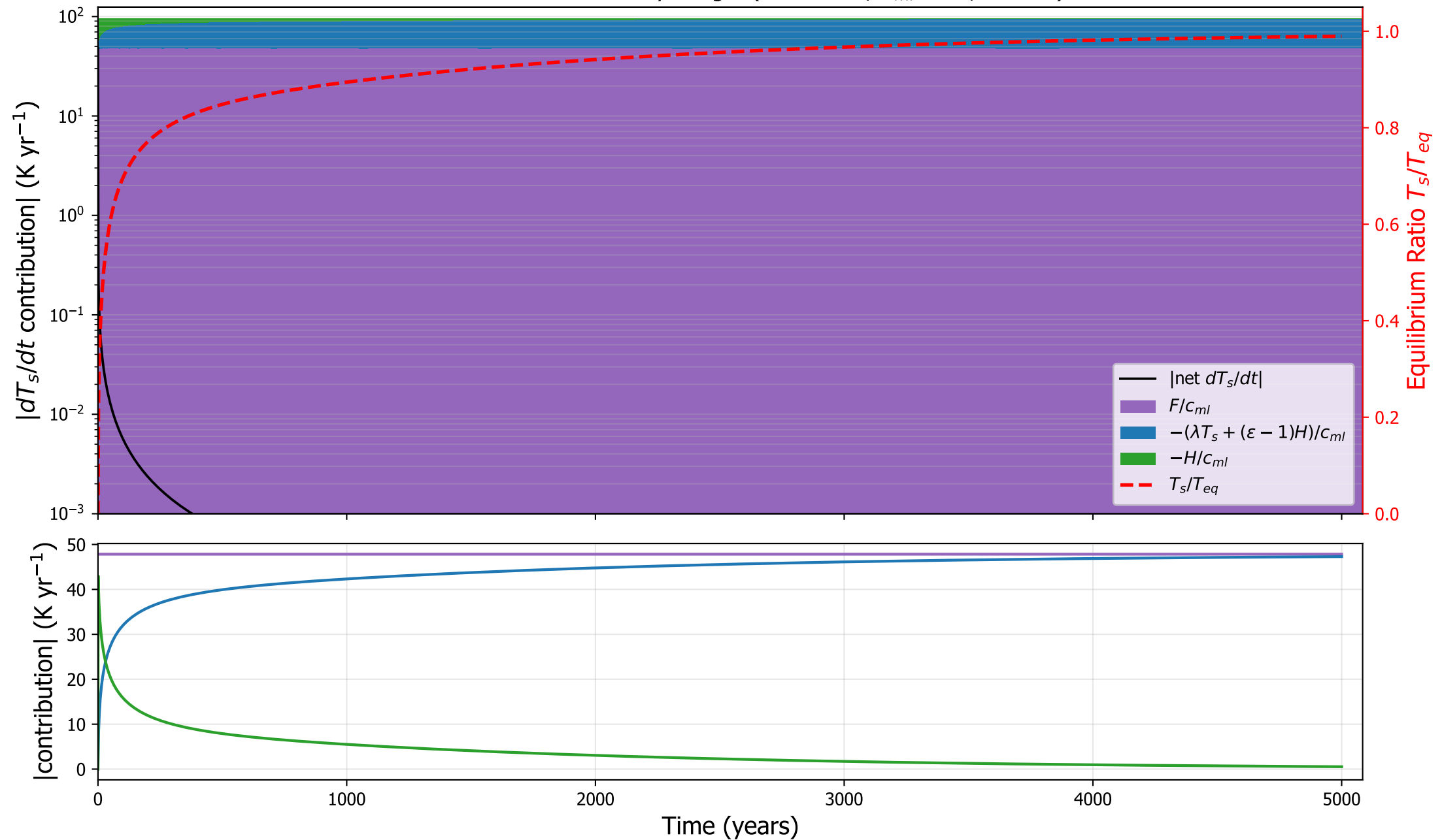
GISSE2R: surface tendency budget ( \kappa=1.5\text{e-}04 , h_{ml}=1 m, \varepsilon=0.92 )
