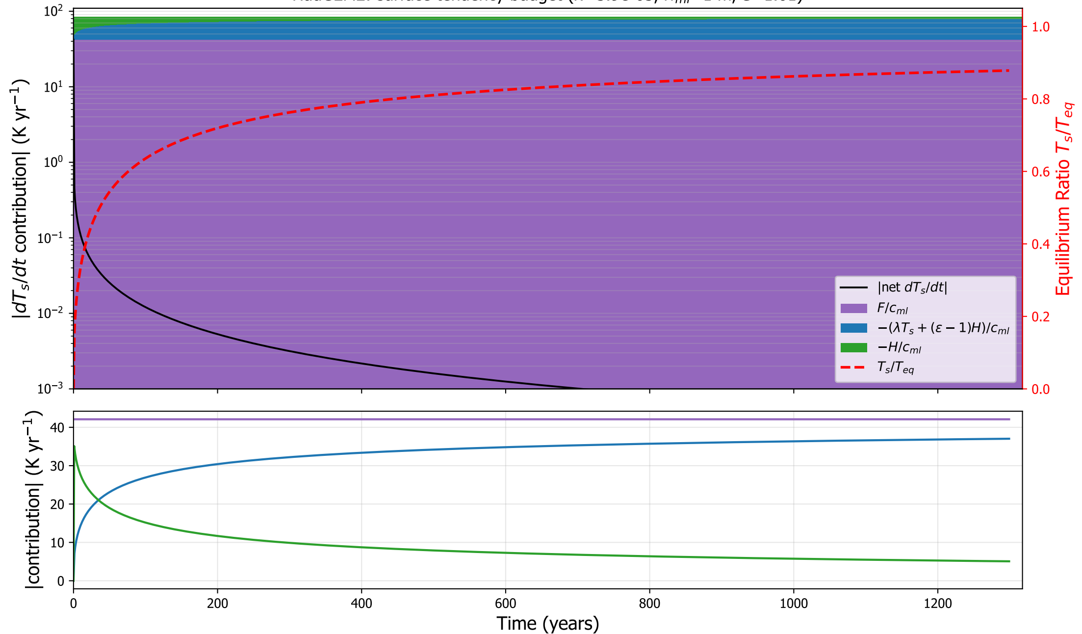
HadGEM2: surface tendency budget ( \kappa=3.9\text{e-}05 , h_{ml}=1 m, \varepsilon=1.01 )
