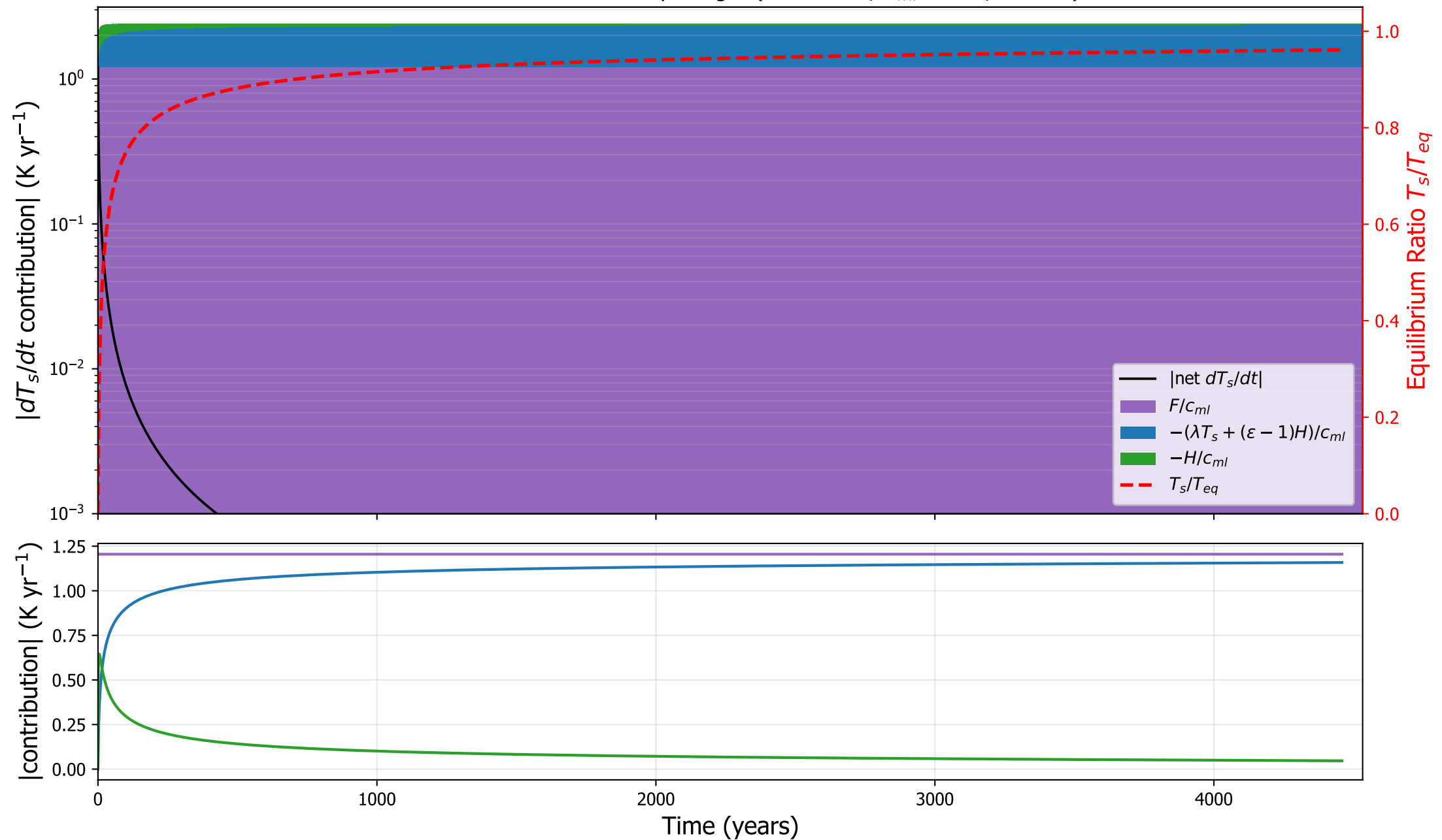
MPIESM11: surface tendency budget ( \kappa=2.9\text{e-}05 , h_{ml}=37 m, \varepsilon=1.00 )
