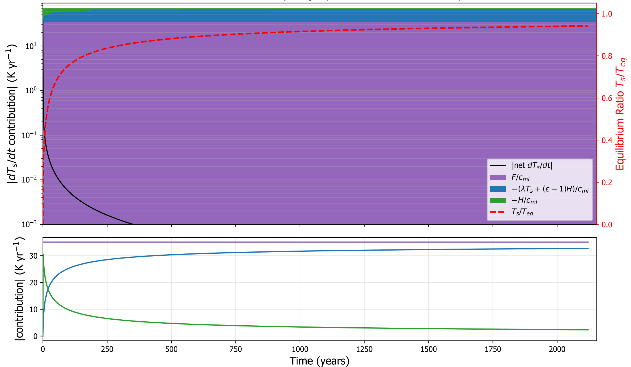
CCSM3: surface tendency budget ( \kappa=4.0\text{e-}05 , h_{ml}=1 m, \varepsilon=0.88 )
