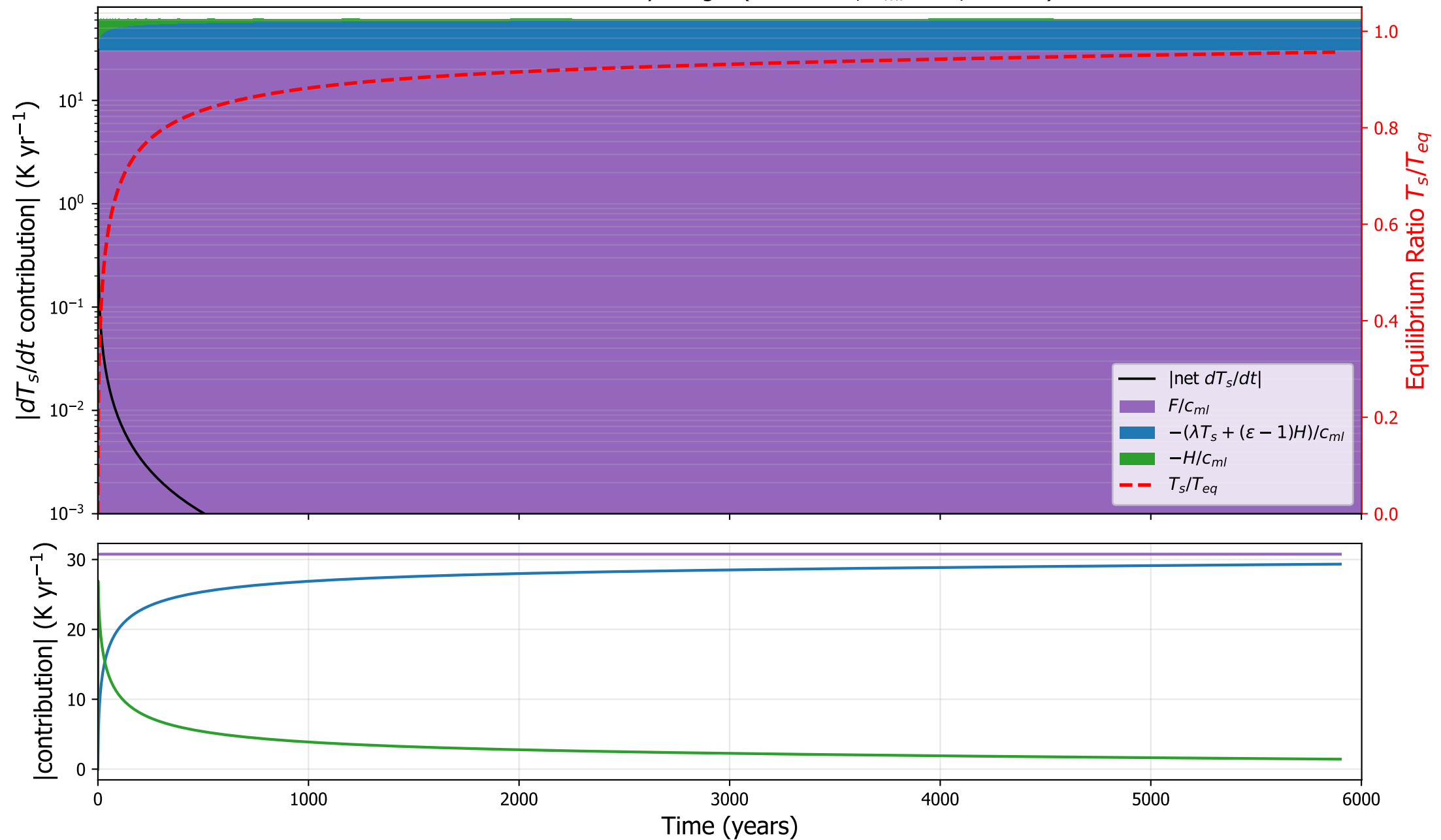
CESM1: surface tendency budget ( \kappa=3.4\text{e-}05 , h_{ml}=1 m, \varepsilon=0.93 )
