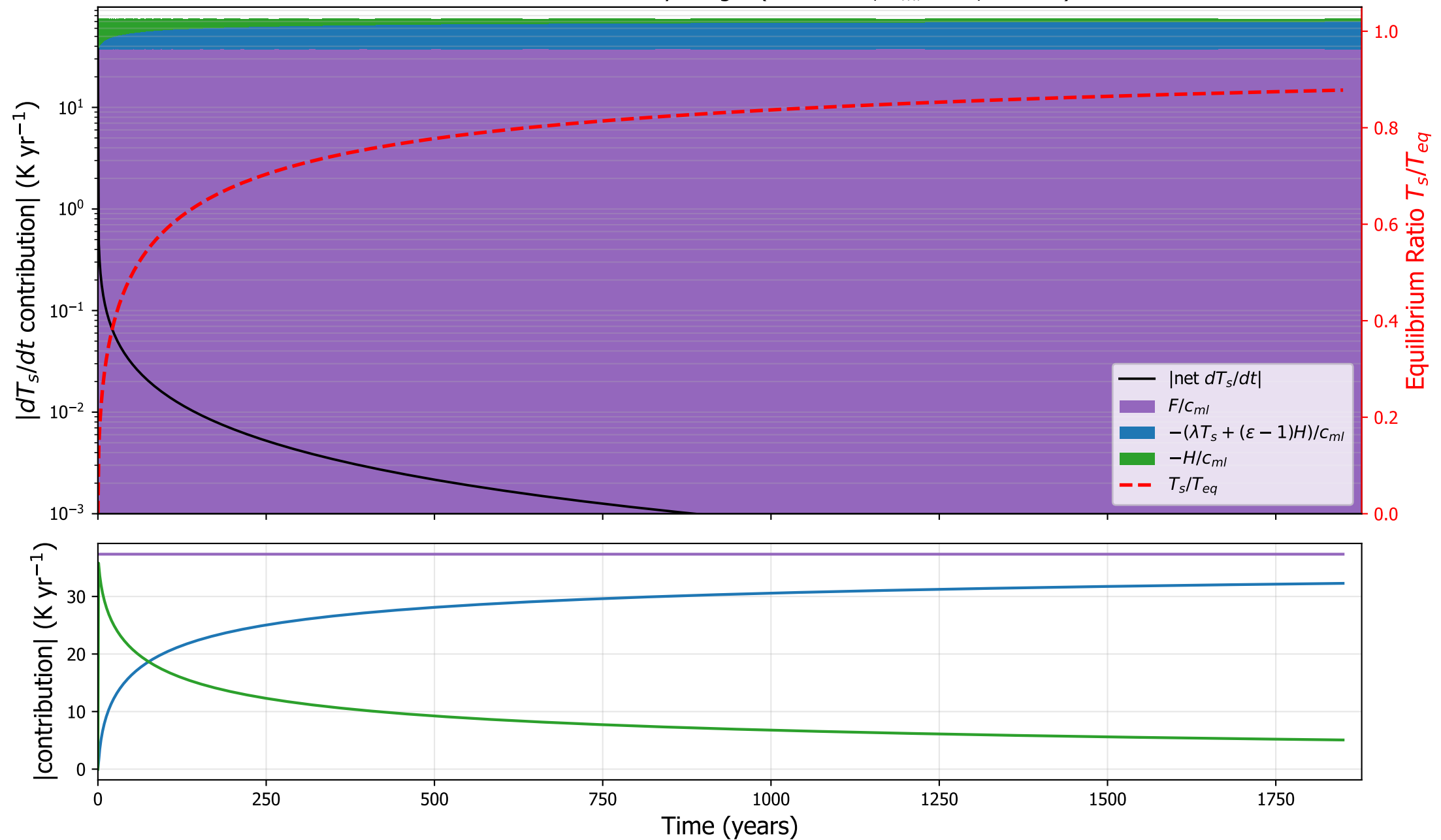
CNRMCM6: surface tendency budget ( \kappa=3.9\text{e-}05 , h_{ml}=1 m, \varepsilon=0.90 )
