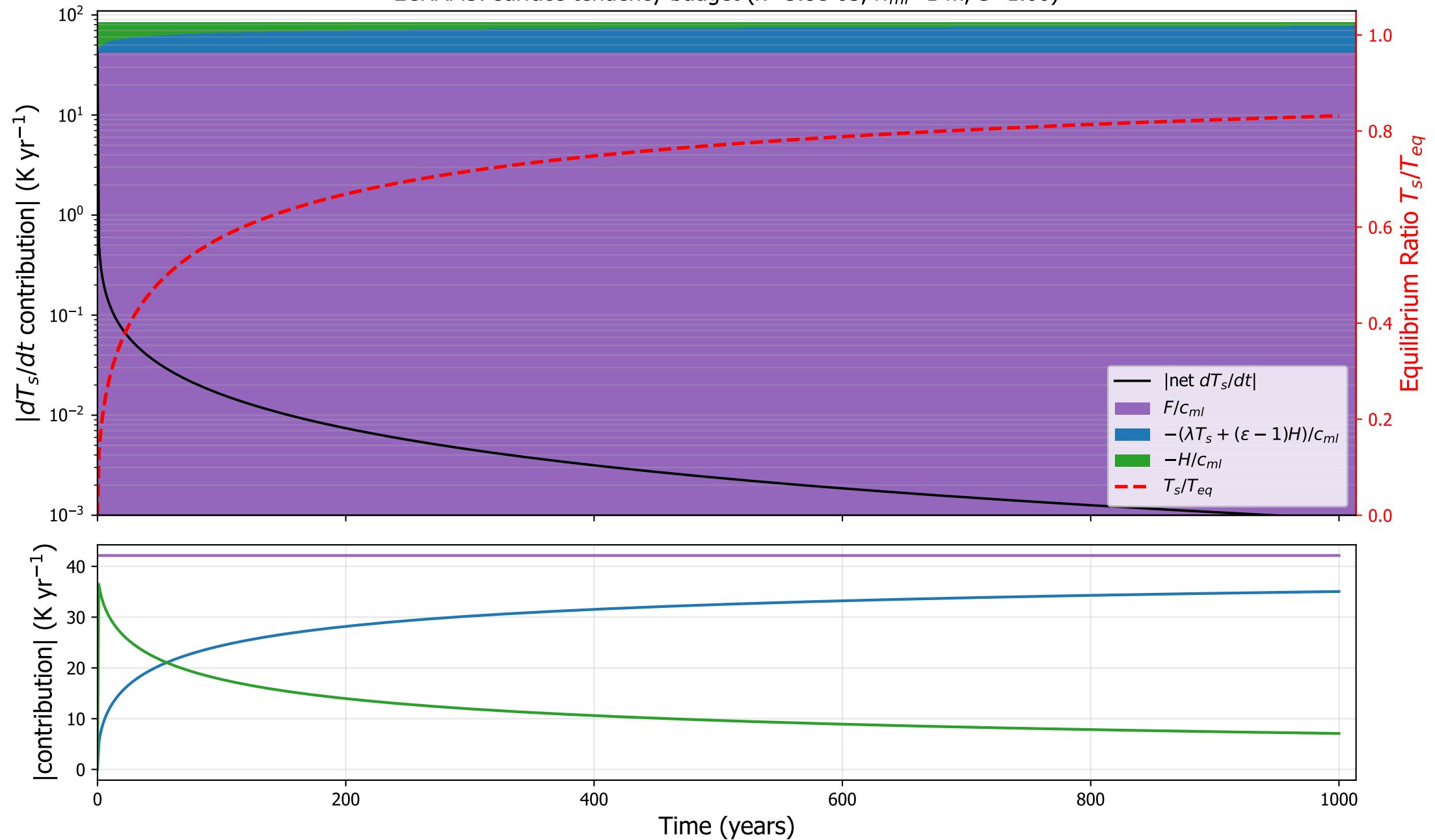
ECHAM5: surface tendency budget ( \kappa=3.8\text{e-}05 , h_{ml}=1 m, \varepsilon=1.00 )
