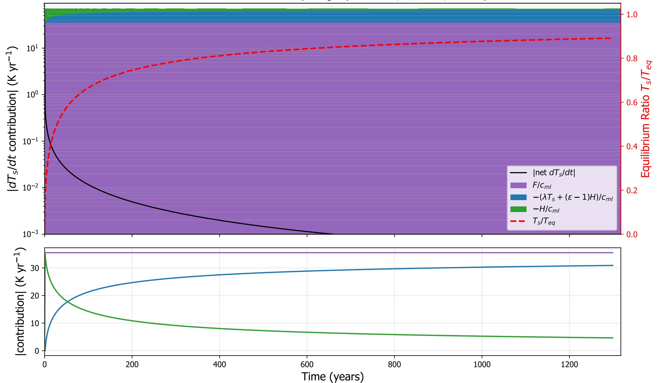
HadGEM2: surface tendency budget ( \kappa=3.2\text{e-}05 , h_{ml}=1\text{ m} , \varepsilon=0.83 )
