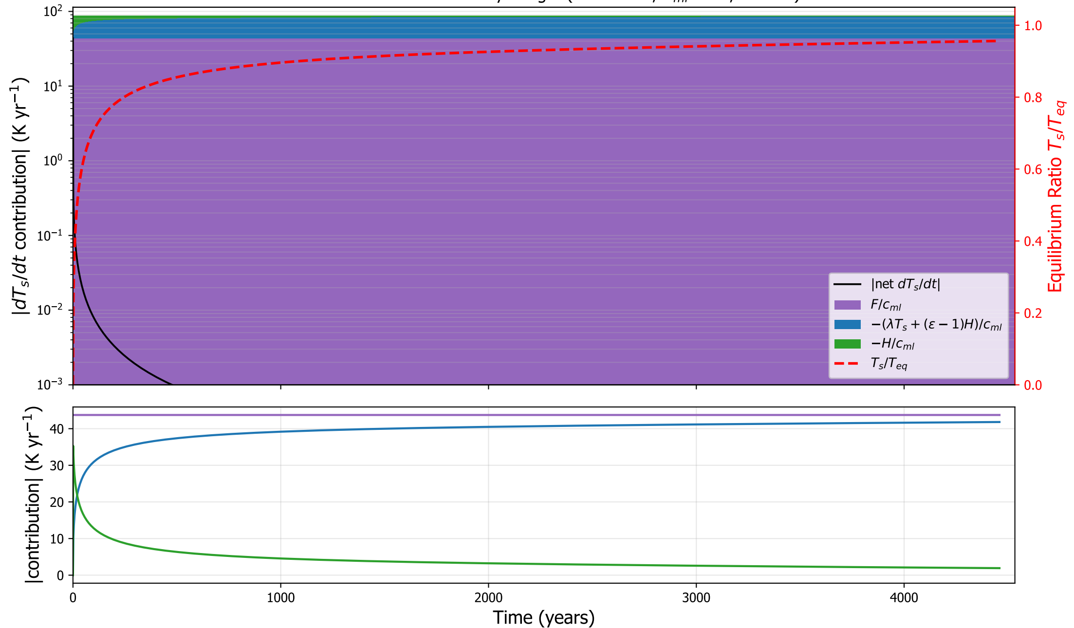
MPIESM11: surface tendency budget ( \kappa=4.5\text{e-}05 , h_{ml}=1 m, \varepsilon=1.00 )
