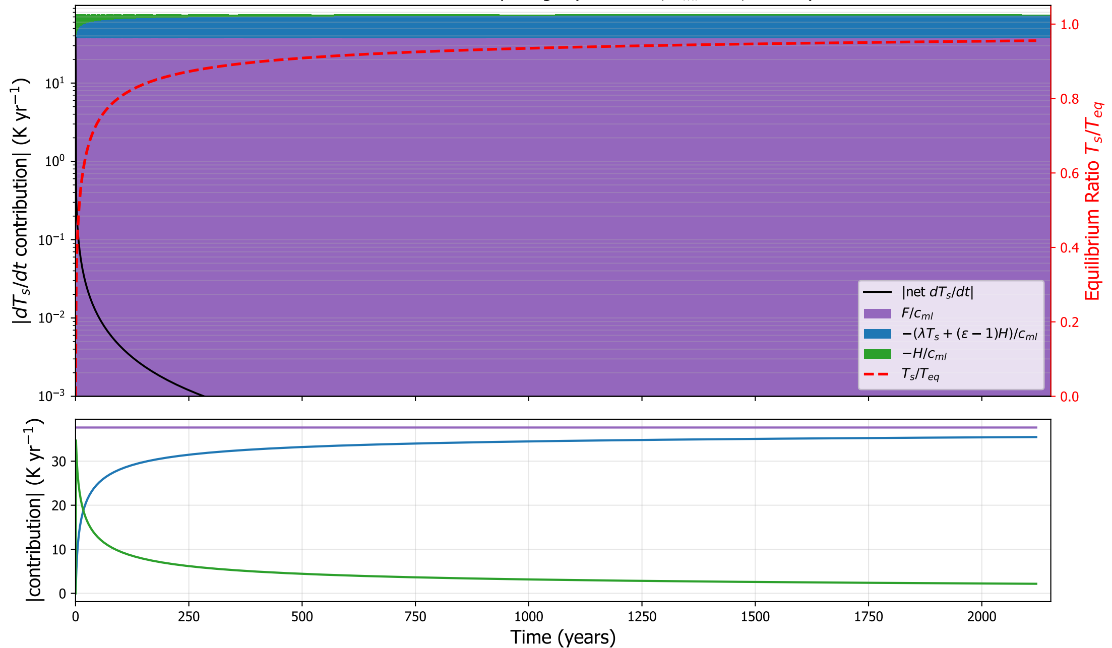
CCSM3: surface tendency budget ( \kappa=4.1\text{e-}05 , h_{ml}=1 m, \varepsilon=0.78 )
