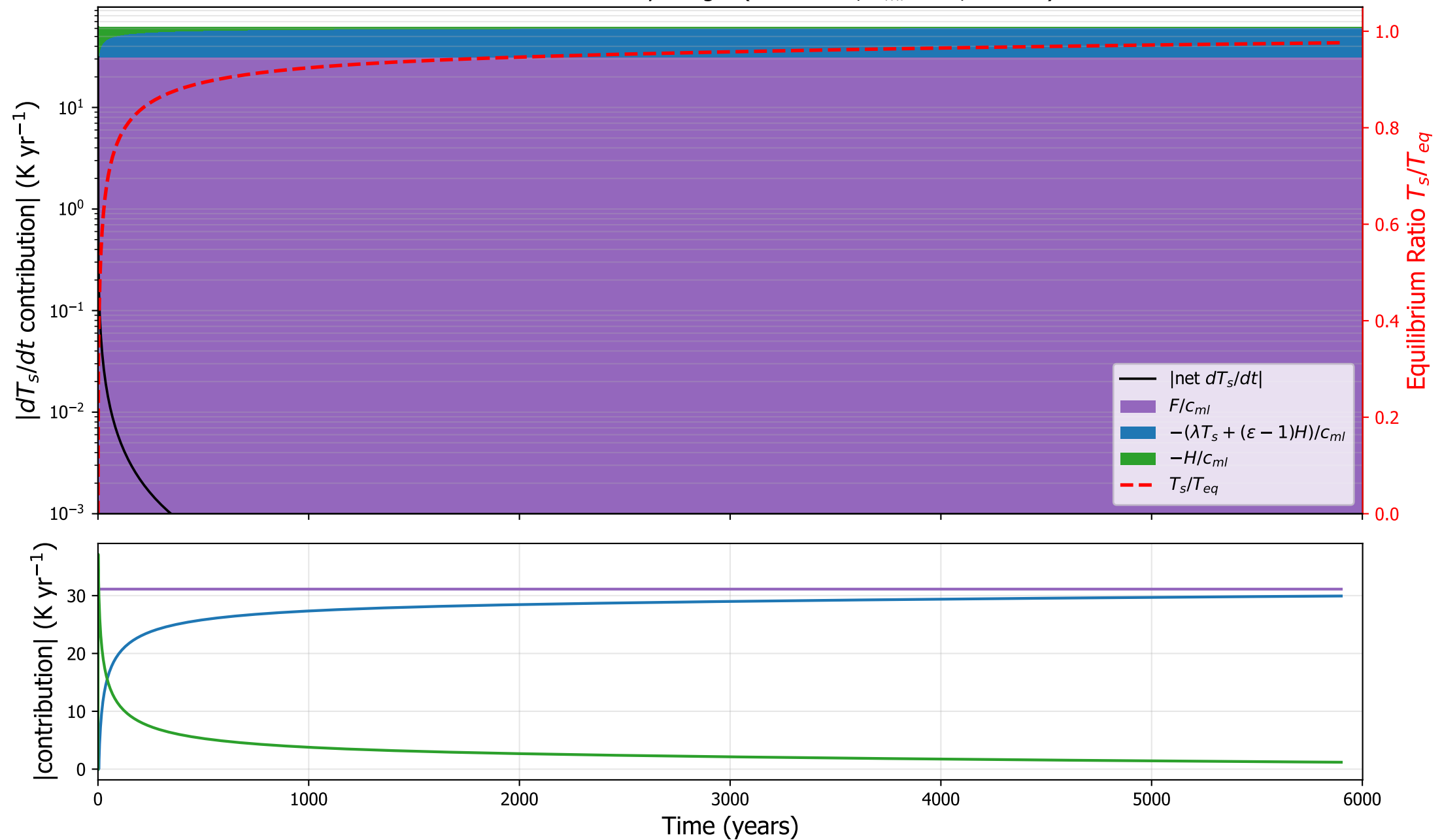
CESM1: surface tendency budget ( \kappa=4.4\text{e-}05 , h_{ml}=1 m, \varepsilon=0.62 )
