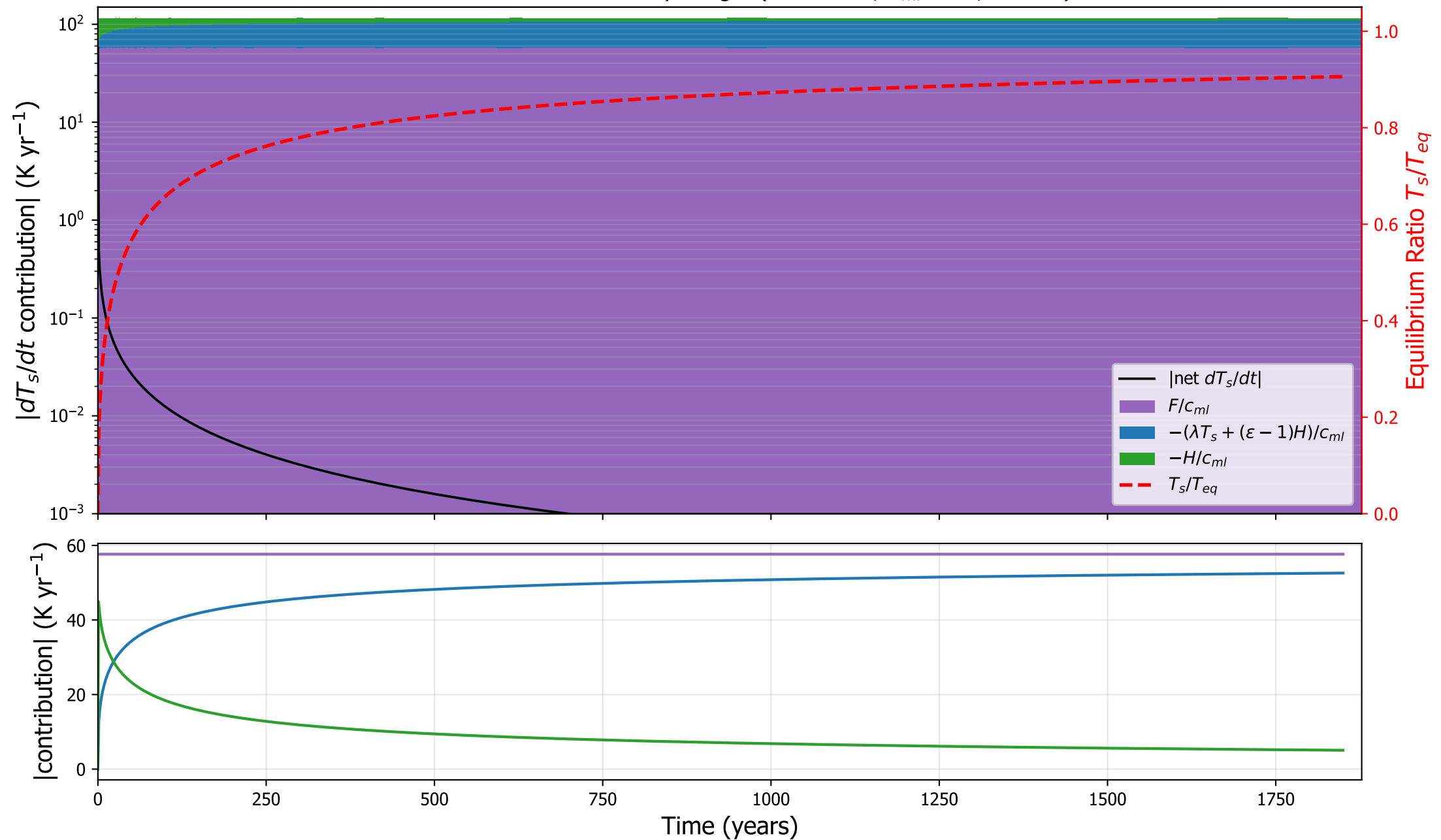
CNRMCM6: surface tendency budget ( \kappa=4.9\text{e-}05 , h_{ml}=1 m, \varepsilon=1.07 )
