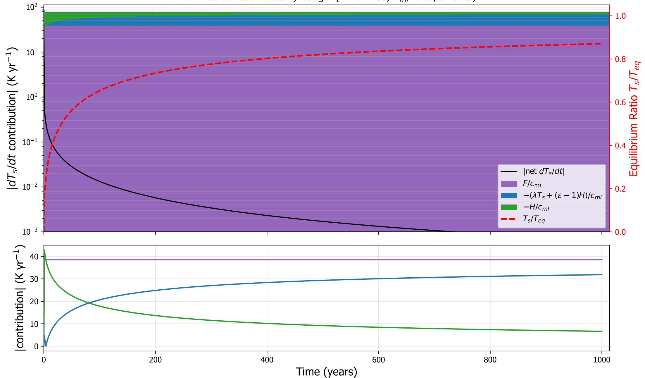
ECHAM5: surface tendency budget ( \kappa=4.2\text{e-}05 , h_{ml}=1 m, \varepsilon=0.75 )
