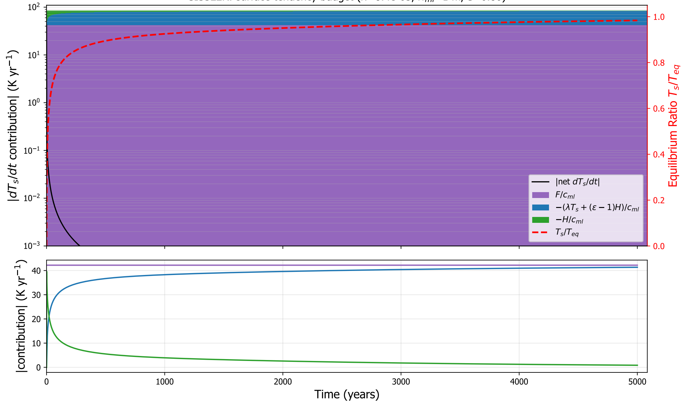
GISSE2R: surface tendency budget ( \kappa=8.4\text{e-}05 , h_{ml}=1 m, \varepsilon=0.80 )
