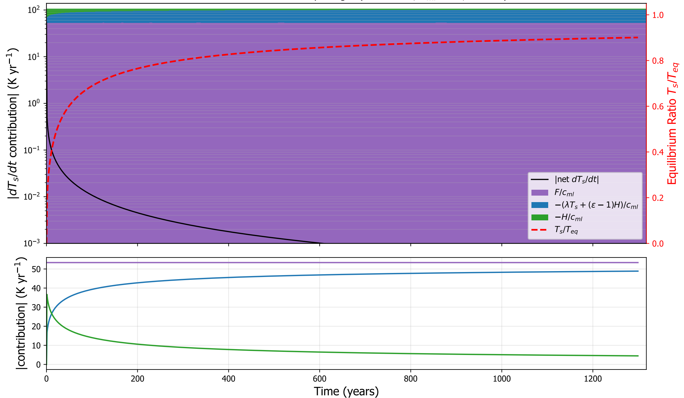
HadGEM2: surface tendency budget ( \kappa=3.3\text{e-}05 , h_{ml}=1 m, \varepsilon=1.18 )
