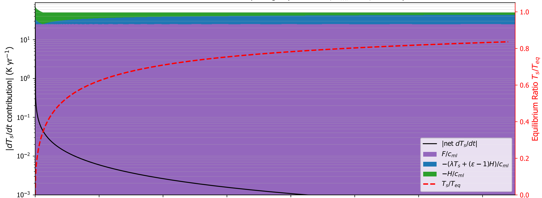
CNRMCM6: surface tendency budget ( \kappa=6.2\text{e-}05 , h_{ml}=1 m, \varepsilon=0.66 )
