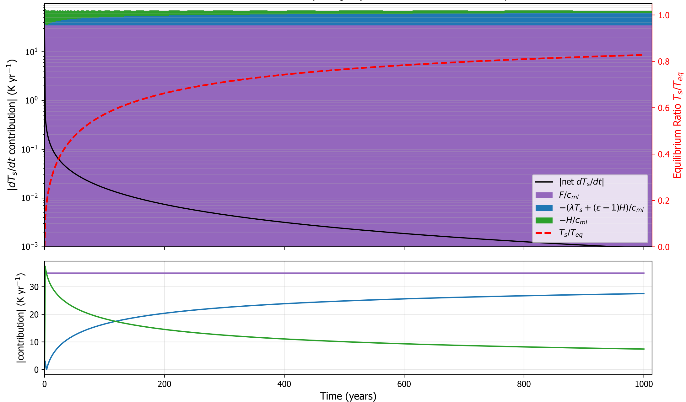
ECHAM5: surface tendency budget ( \kappa=4.2\text{e-}05 , h_{ml}=1 m, \varepsilon=0.81 )
