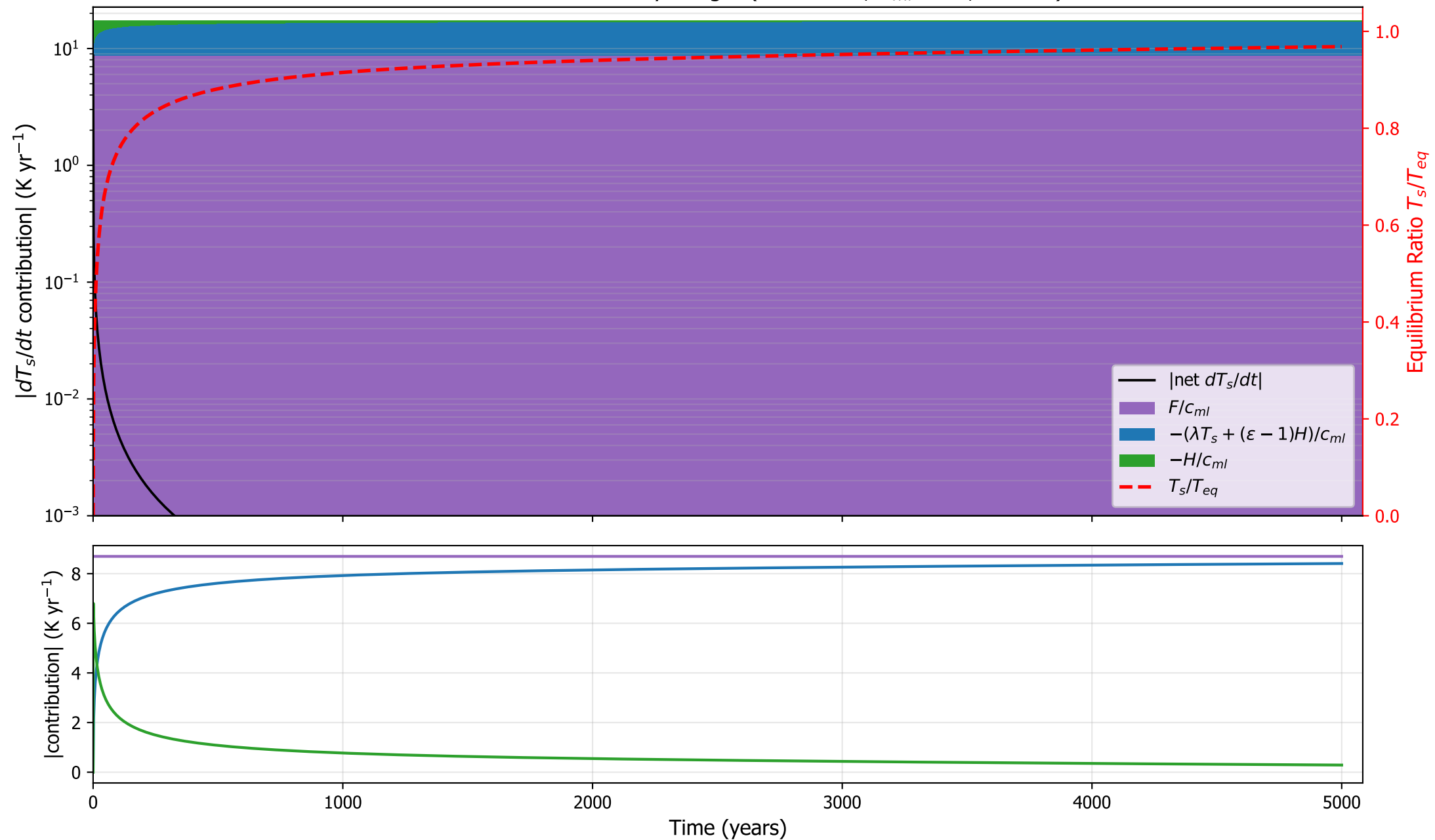
GISSE2R: surface tendency budget ( \kappa=4.5\text{e-}05 , h_{ml}=4 m, \varepsilon=0.96 )
