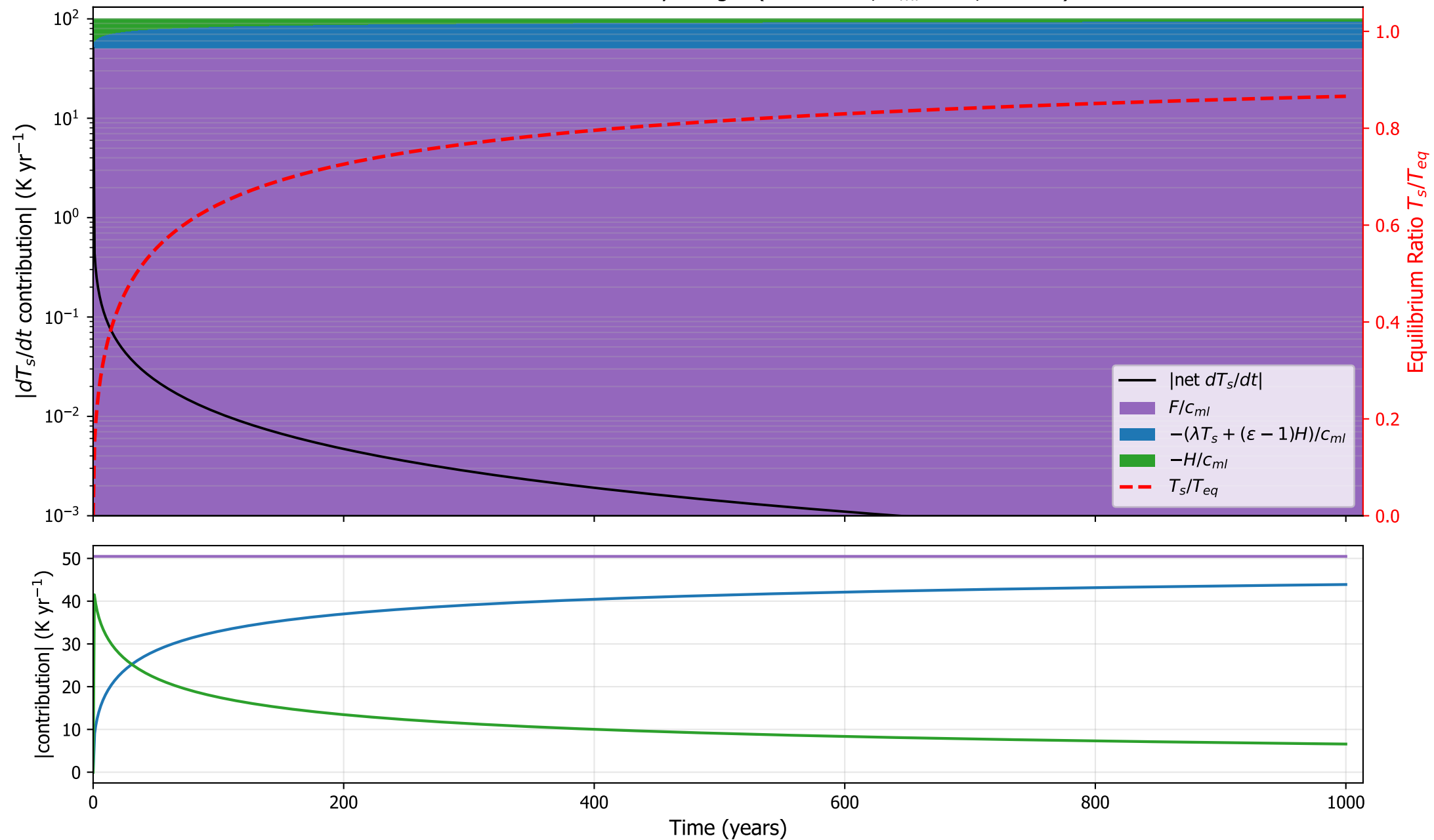
IPSLCM5A: surface tendency budget ( \kappa=6.4\text{e-}05 , h_{ml}=1 m, \varepsilon=1.03 )
