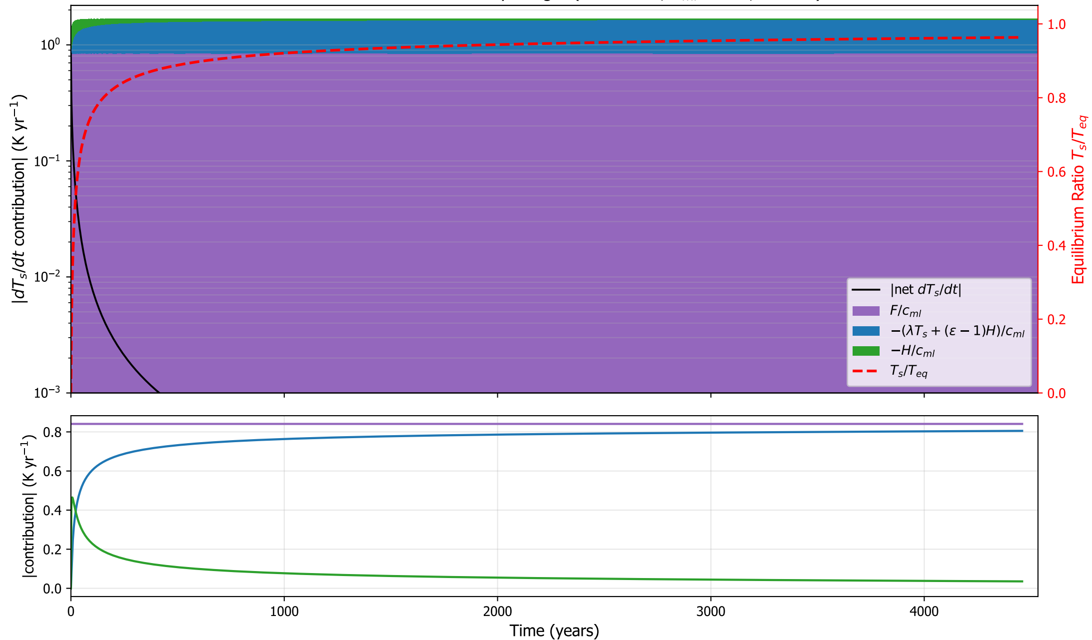
MPIESM11: surface tendency budget ( \kappa=2.9\text{e-}05 , h_{ml}=48 m, \varepsilon=0.86 )
