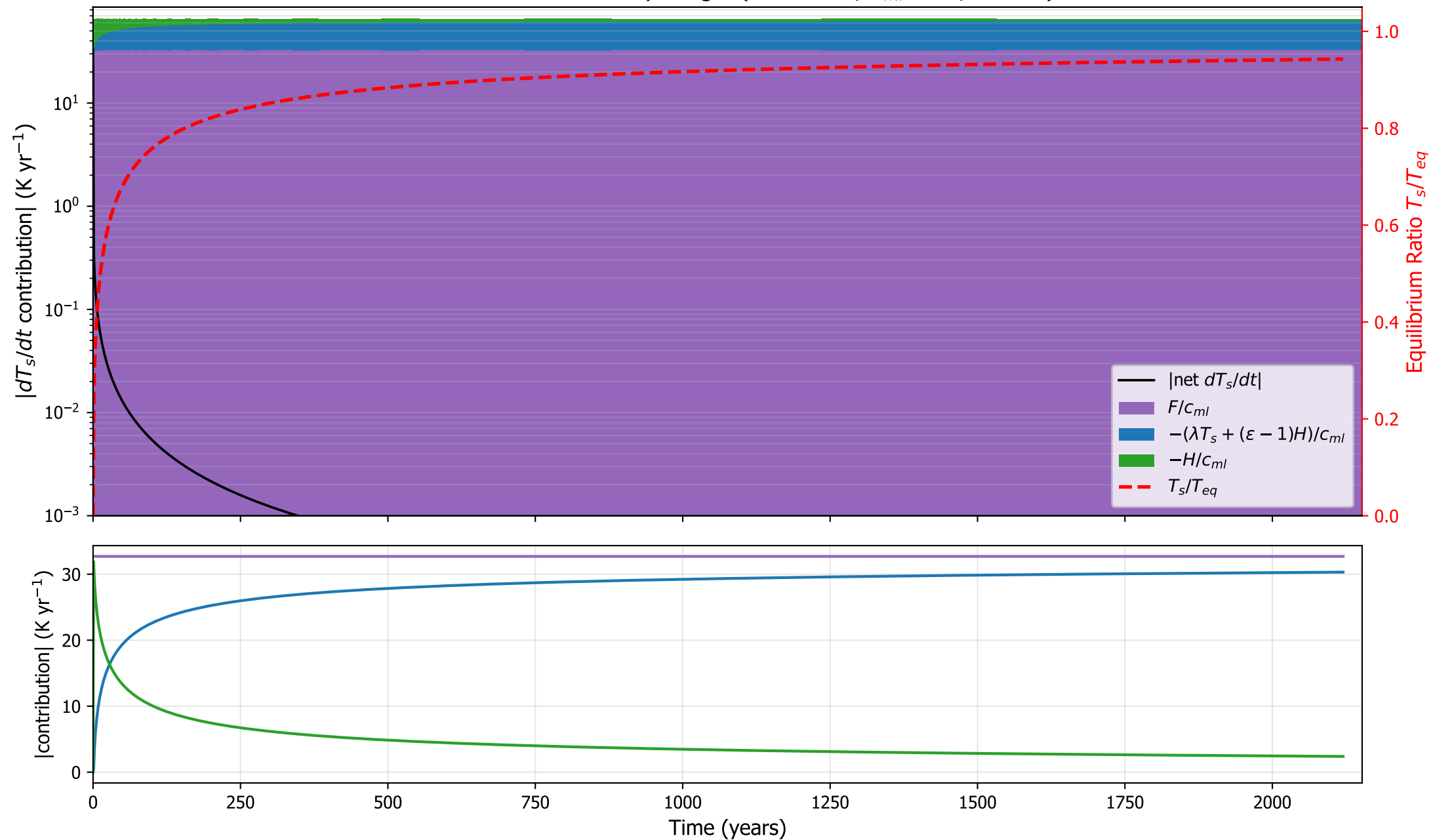
CCSM3: surface tendency budget ( \kappa=4.3\text{e-}05 , h_{ml}=1 m, \varepsilon=0.78 )
