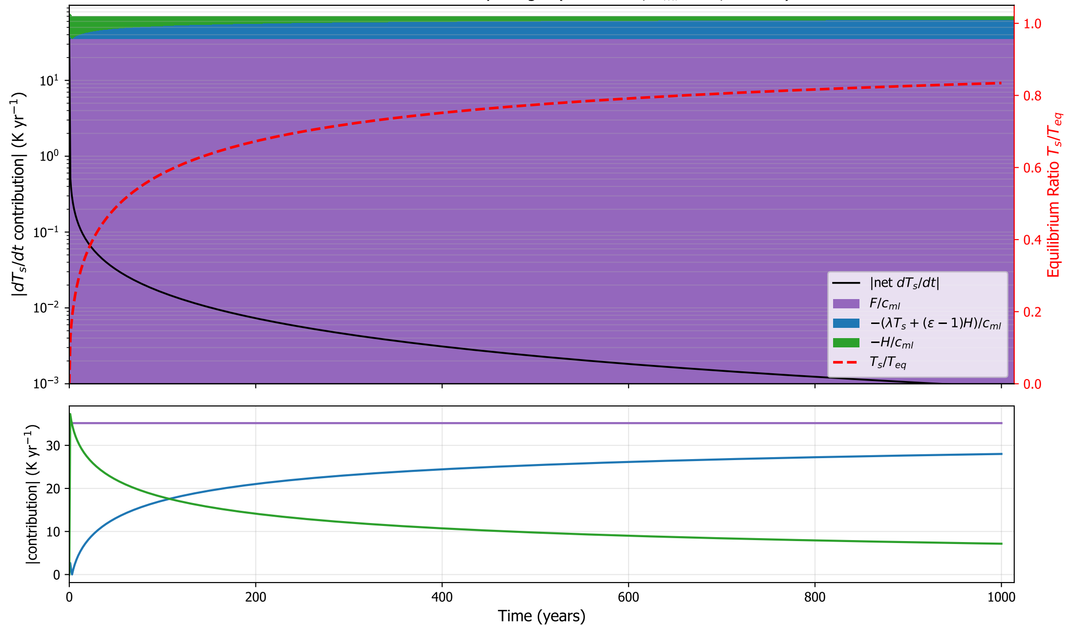
ECHAM5: surface tendency budget ( \kappa=3.9\text{e-}05 , h_{ml}=1 m, \varepsilon=0.81 )
