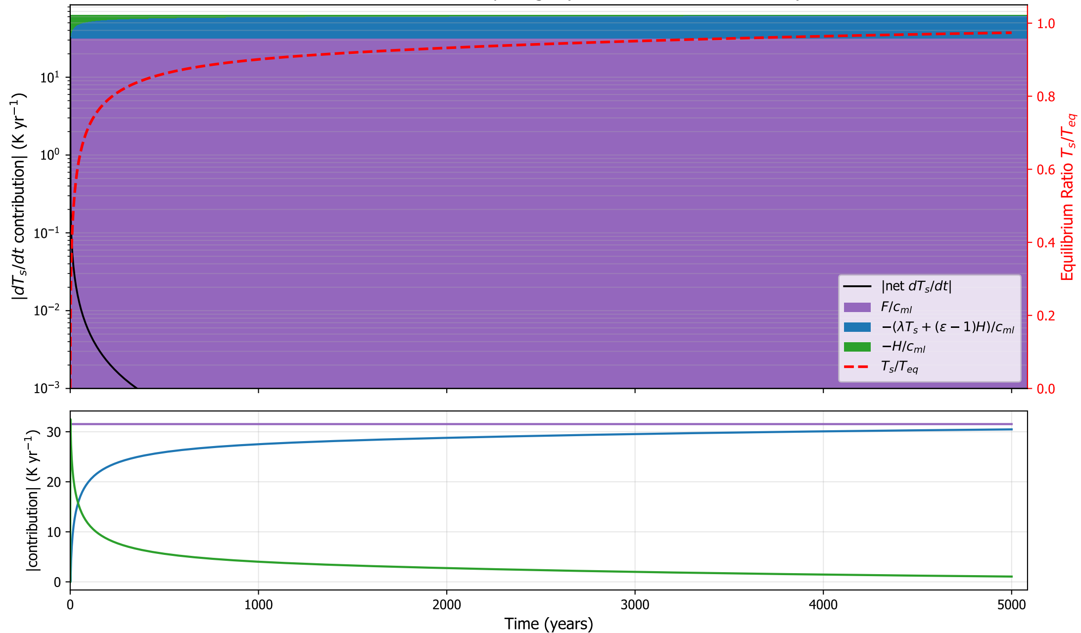
GISSE2R: surface tendency budget ( \kappa=7.4\text{e-}05 , h_{ml}=1 m, \varepsilon=0.78 )
