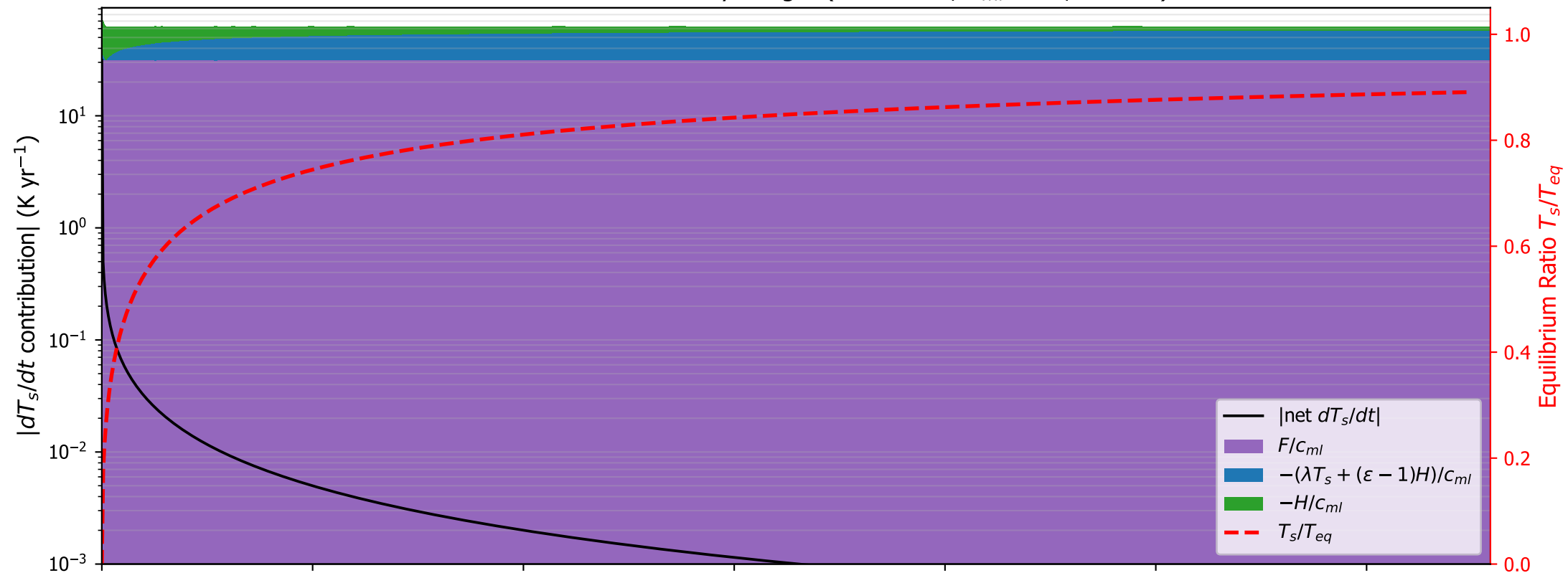
HadGEM2: surface tendency budget ( \kappa=3.3\text{e-}05 , h_{ml}=1 m, \varepsilon=0.73 )
