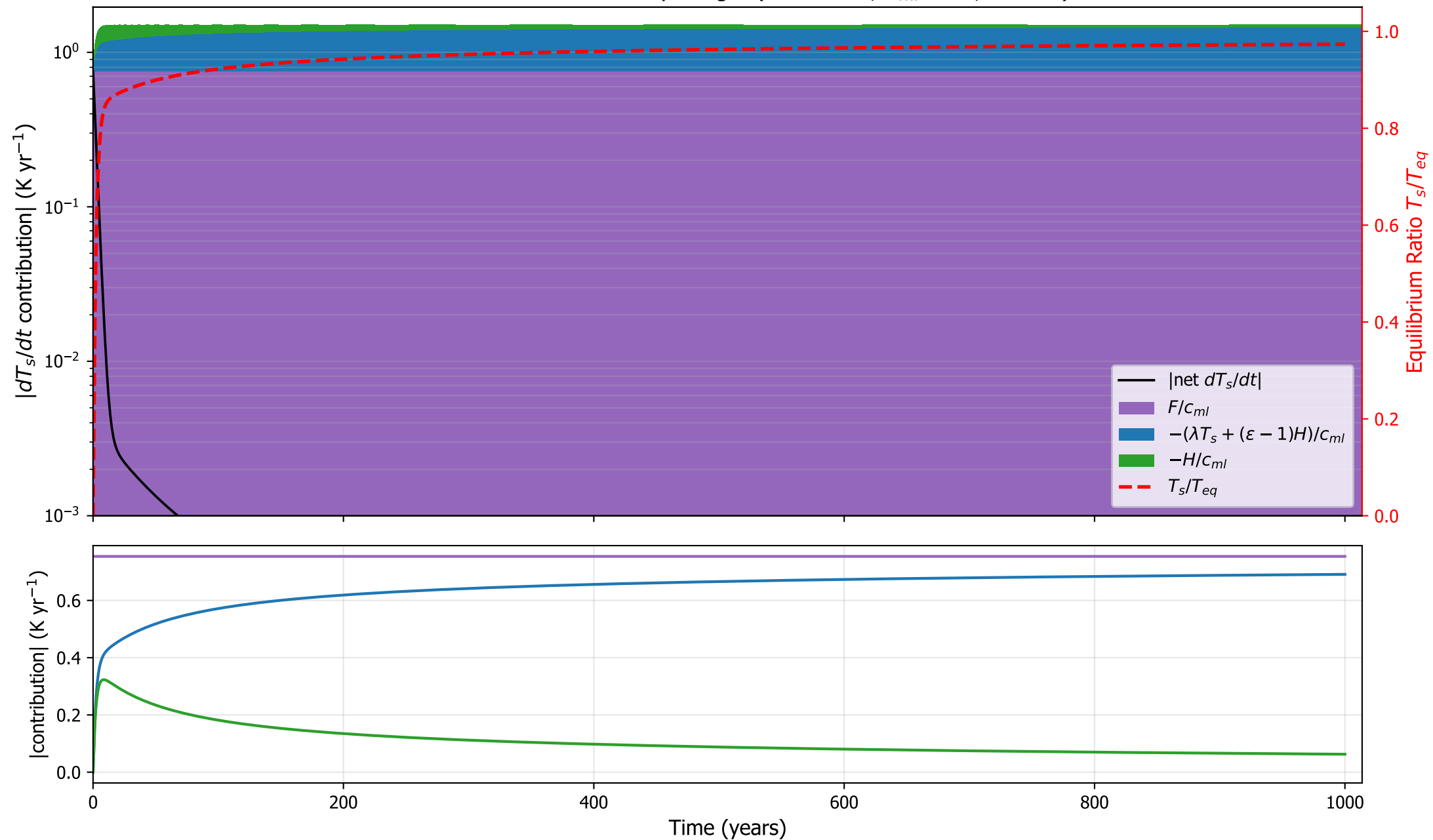
IPSLCM5A: surface tendency budget ( \kappa=1.0\text{e-}07 , h_{ml}=1 m, \varepsilon=0.32 )
