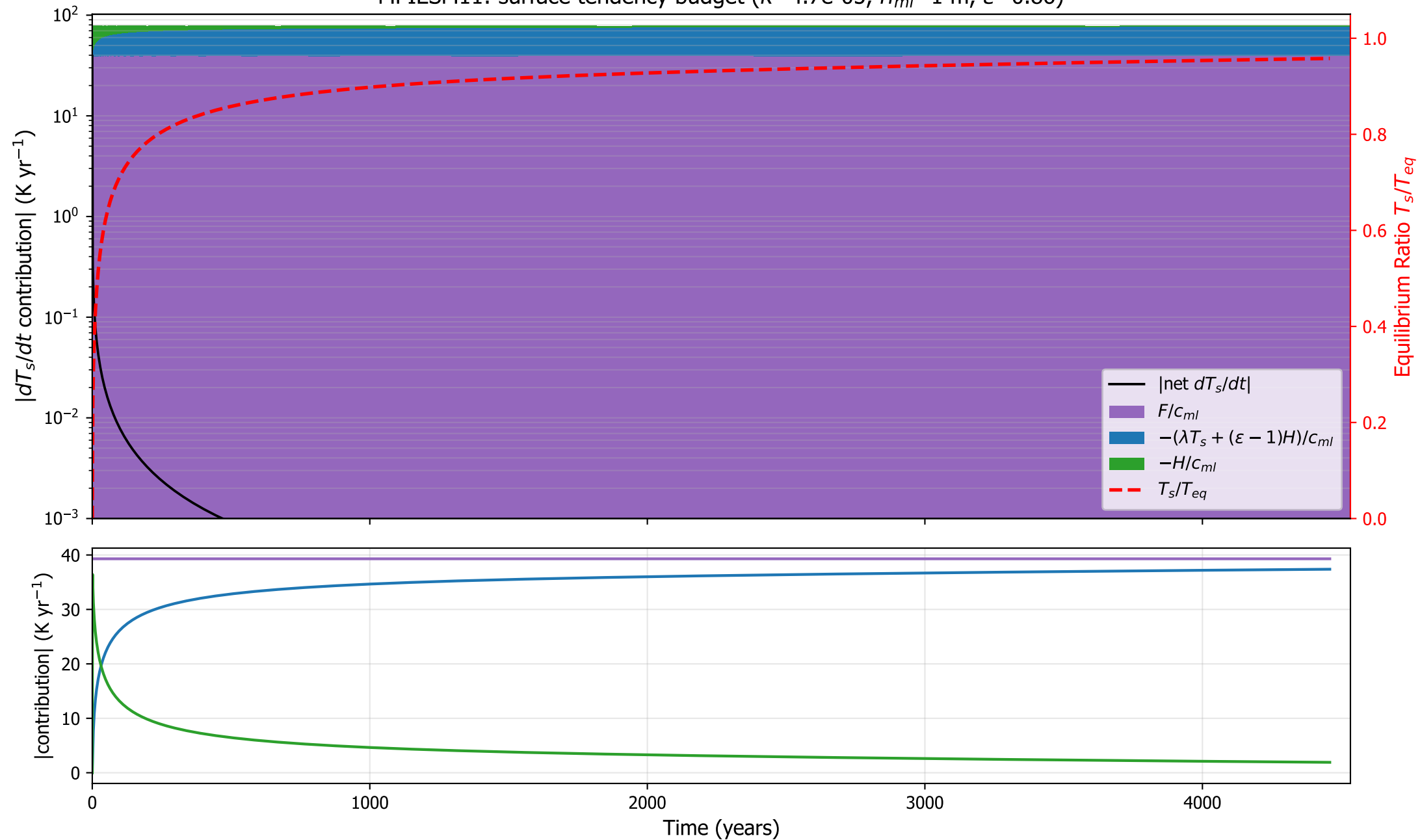
MPIESM11: surface tendency budget ( \kappa=4.7\text{e-}05 , h_{ml}=1 m, \varepsilon=0.86 )
